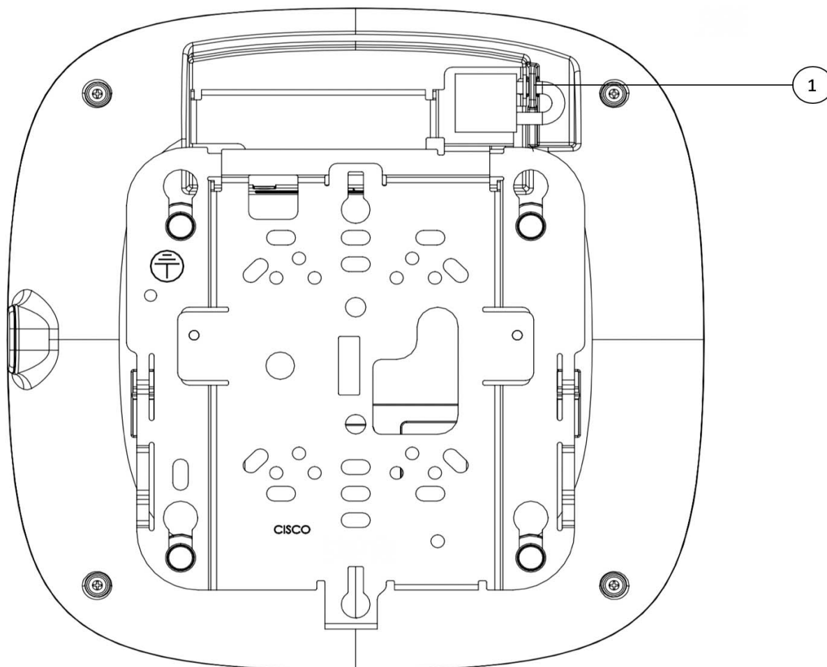
Figure 6 Locking the AP to the Bracket
