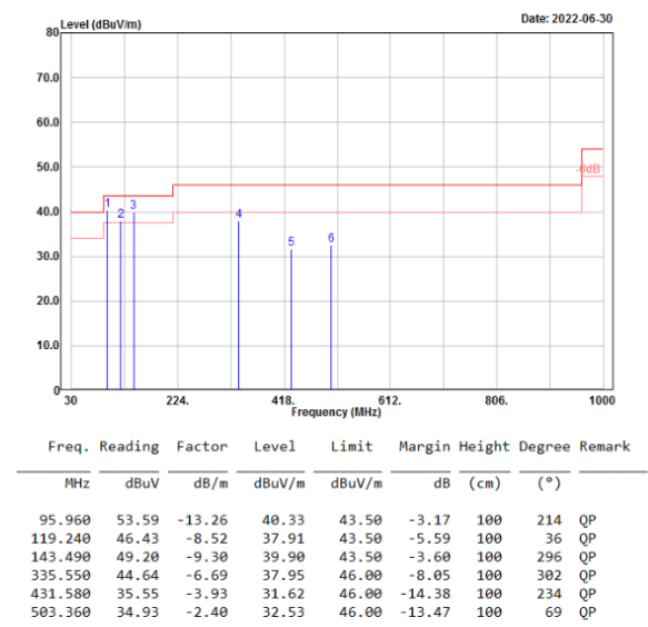
Mode 4 / Vertical
