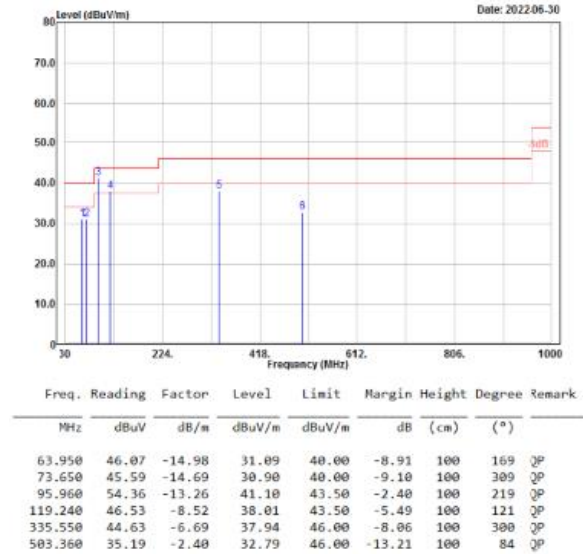
Mode 3 / Vertical
