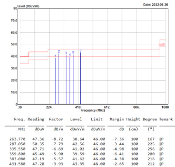
Mode 3 / Horizontal
