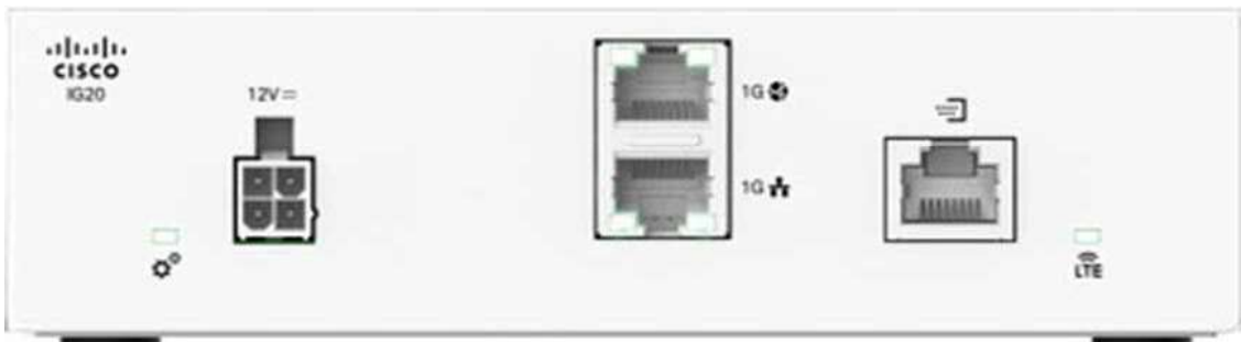
Figure 10 IoT Gateway IG21 Front Panel
