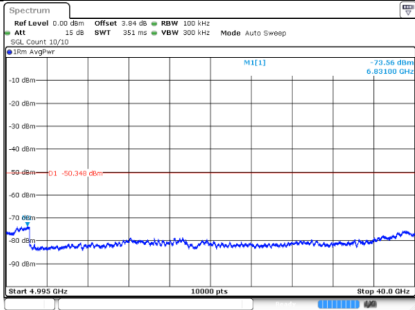
4950-10MHz-802.11ac-1-b
