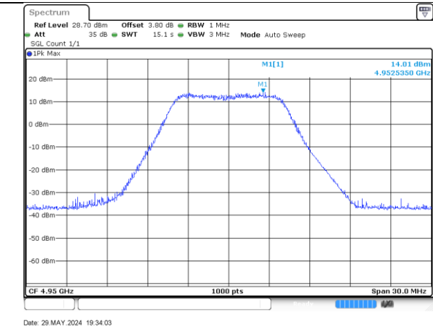
4950MHz-10MHz-802.11a-1-b
