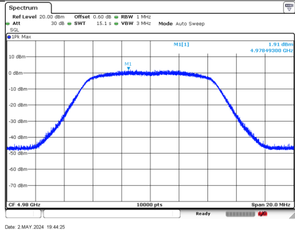
4980MHz-10MHz-802.11n-1-b
