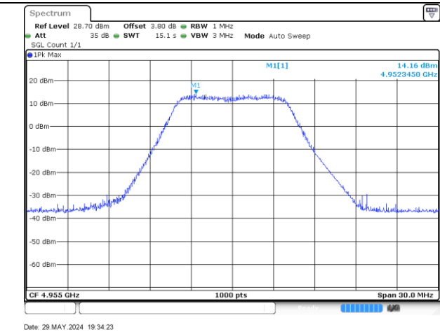
4955MHz-10MHz-802.11a-1-b
