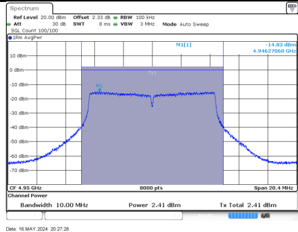
4950-10MHz-802.11ac-2-b
