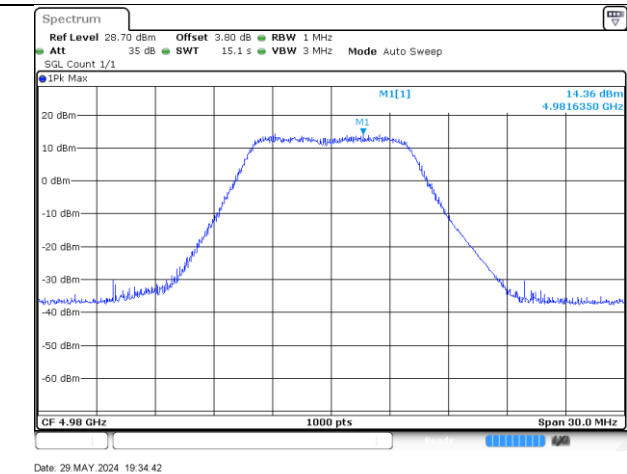
4980MHz-10MHz-802.11a-1-b
