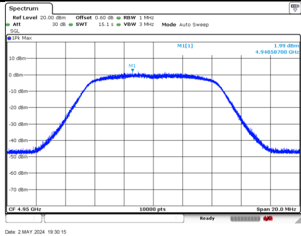
4950MHz-10MHz-802.11ac-1-b
