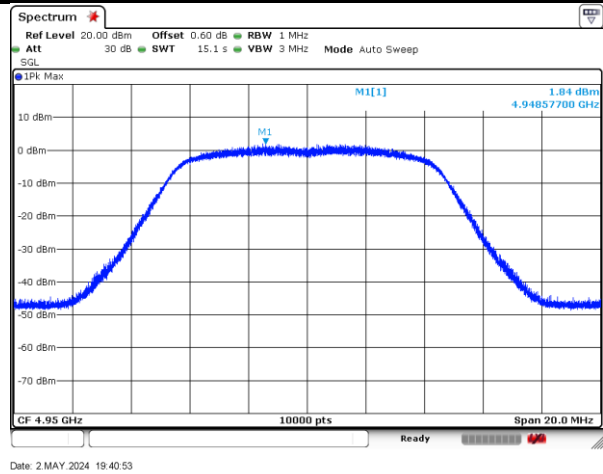
4950MHz-10MHz-802.11n-1-b
