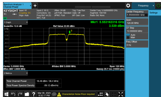
Antenna B
