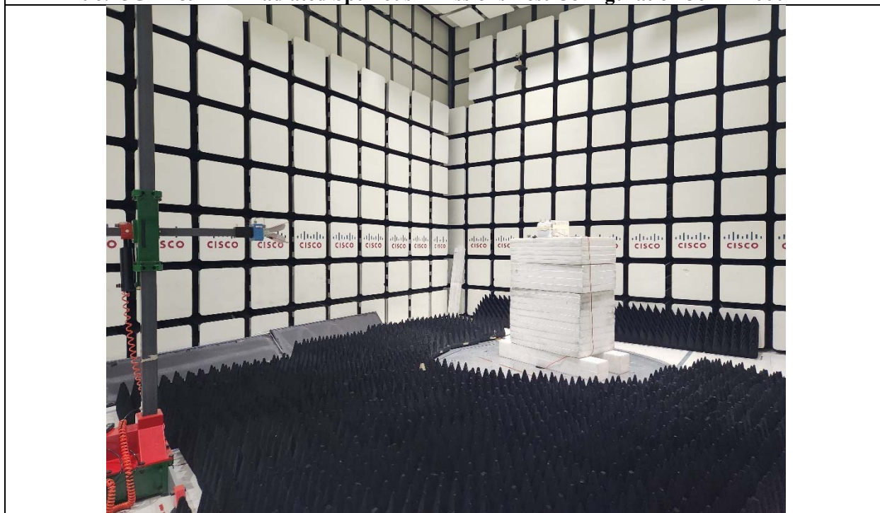
Title: 5GHz Radiated Spurious Emissions Test Configuration 1GHz - 18GHz
