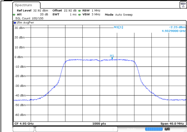
4950MHz-tx2-cobalt_10
