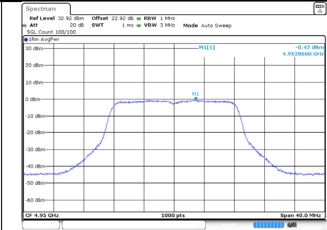
4950MHz-tx2-cobalt_12
