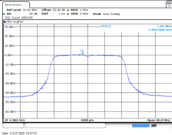
4965MHz-tx2-pine_11
