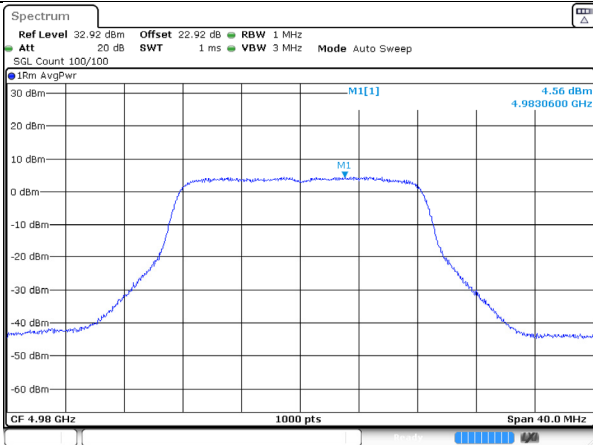
4980MHz-tx2-cobalt_11
