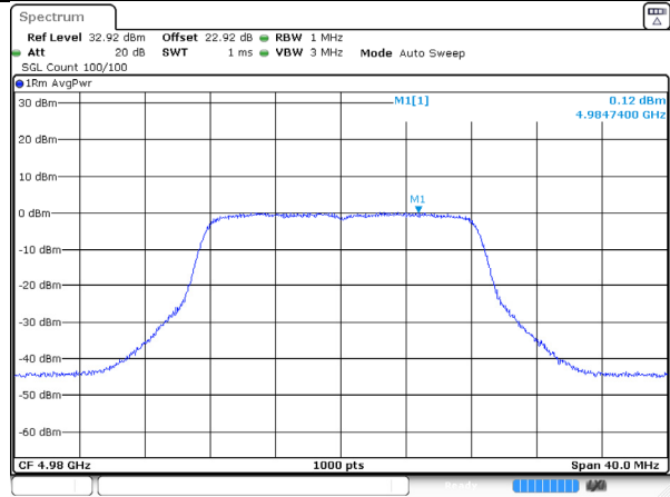
4980MHz-tx2-cobalt_13
