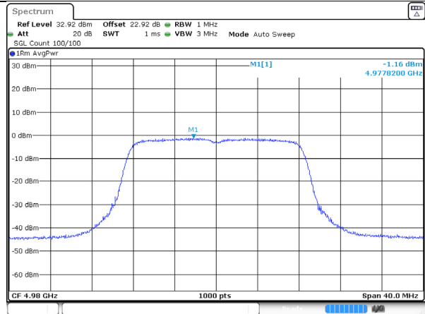
4980MHz-tx2-cobalt_13
