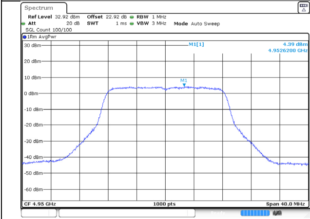
4950MHz-tx2-cobalt_10
