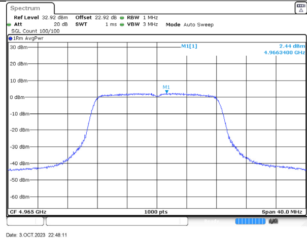
4965MHz-tx2-pine_13
