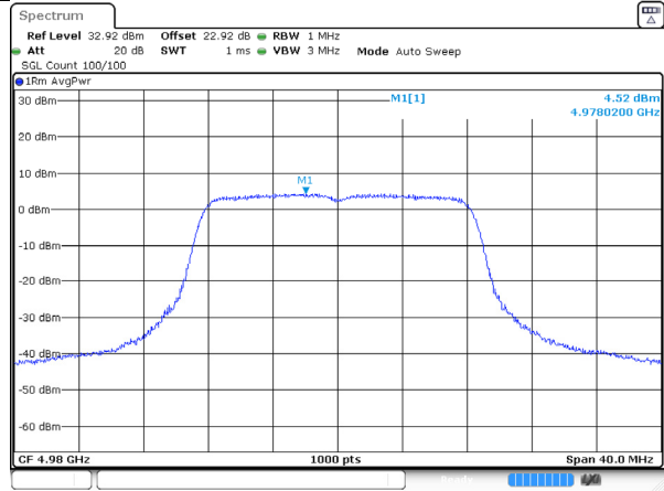
4980MHz-tx2-pine_10
