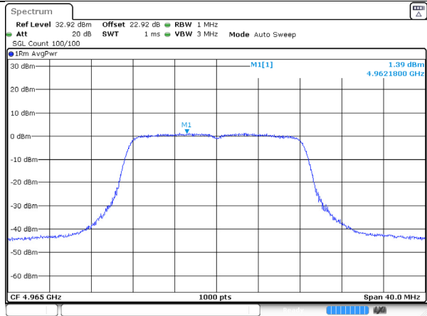
4965MHz-tx1-pine_10
