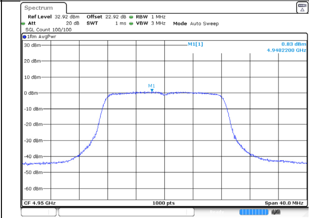
4950MHz-tx2-cobalt_12
