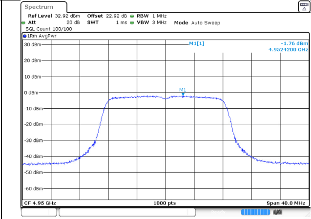
4950MHz-tx2-pine_11
