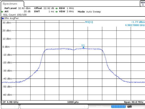
4980MHz-tx2-cobalt_11
