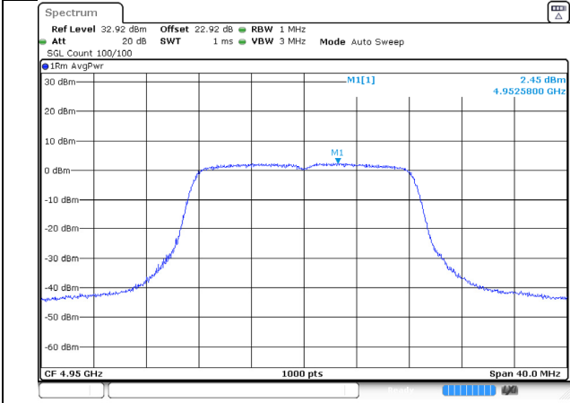
4950MHz-tx2-cobalt_16
