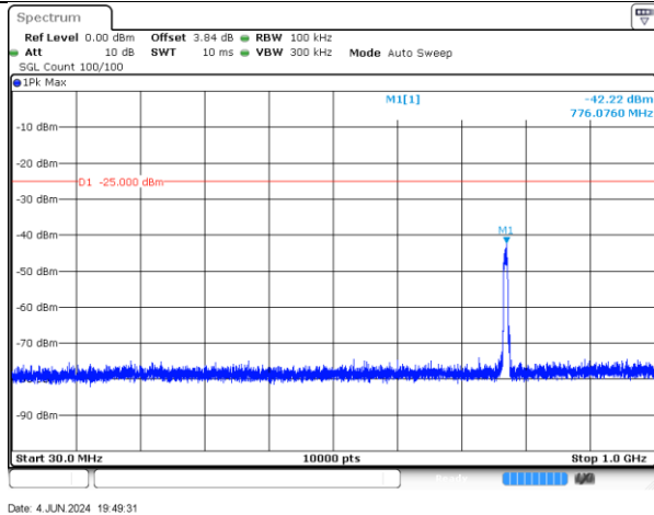
4980-10MHz-802.11a-1-b
