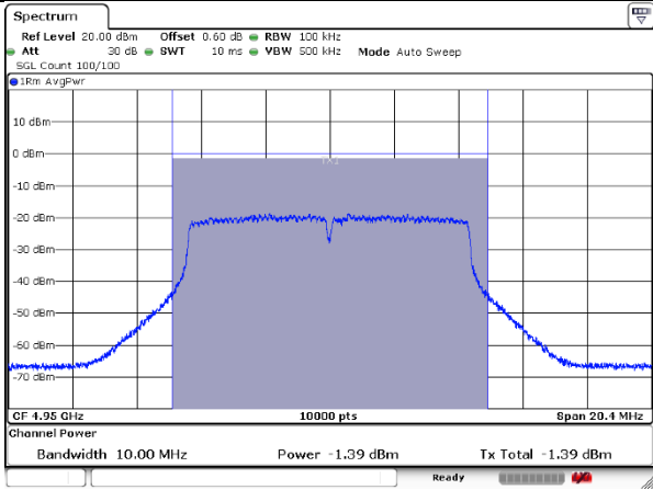
4950MHz-10MHz-802.11ac-1-b
