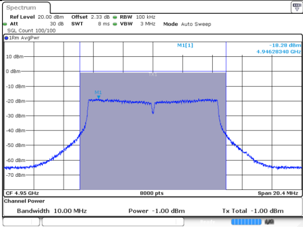
4950MHz-10MHz-802.11n-1-b
