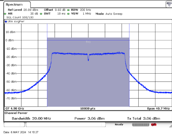
4980MHz-20MHz-802.11ac-1-b
