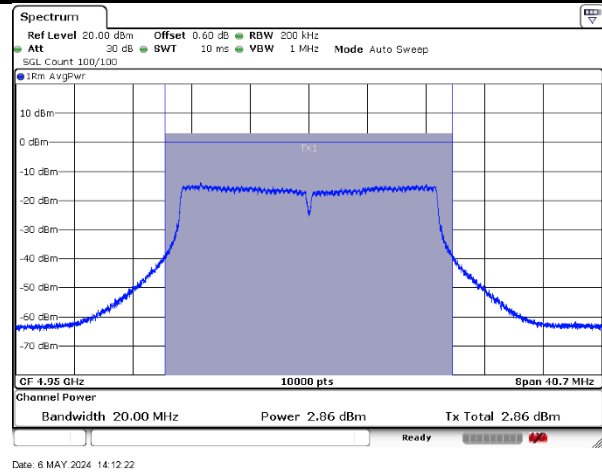
4950MHz-20MHz-802.11ac-1-b
