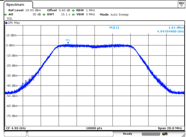
4950-10MHz-802.11ac-1-b
