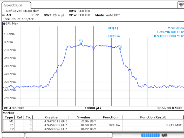
4950MHz-10MHz-802.11n-Radio_1
