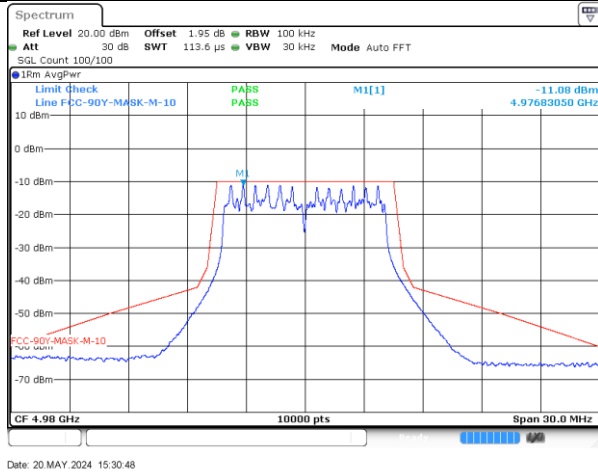
4980MHz-10MHz-802.11a-Radio_1
