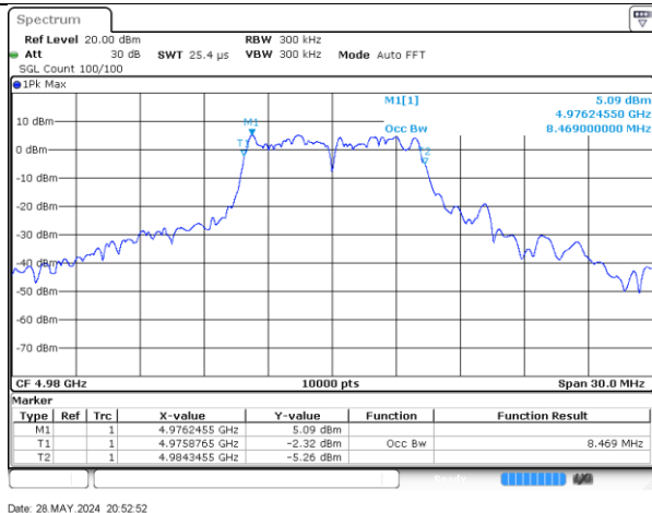
4980MHz-10MHz-802.11a-Radio_2
