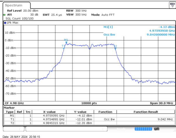
4980MHz-10MHz-802.11n-Radio_2
