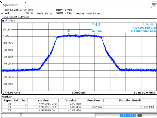
4950MHz-20MHz-802.11n-Radio_1
