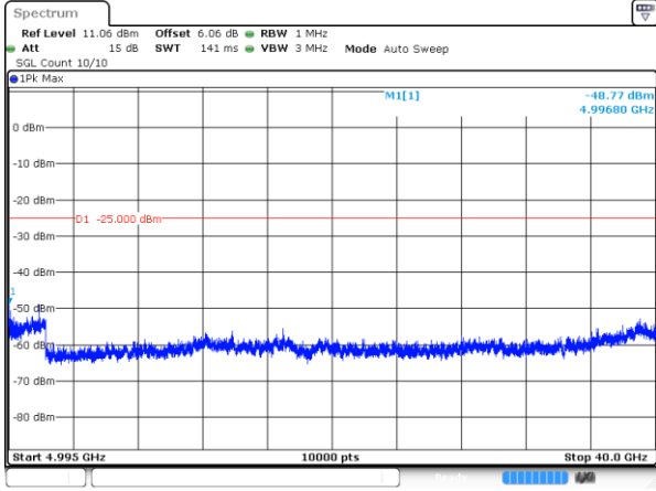
4980-10MHz-802.11a-2-b
