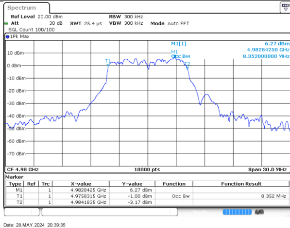
4980-10MHz-802.11a-Radio_1
