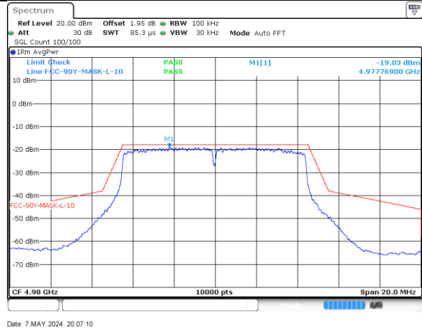
4980MHz-10MHz-802.11n-Radio_1
