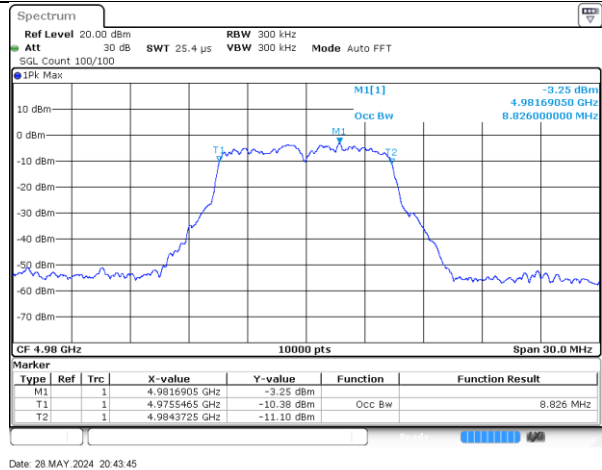
4980-10MHz-802.11n-Radio_1
