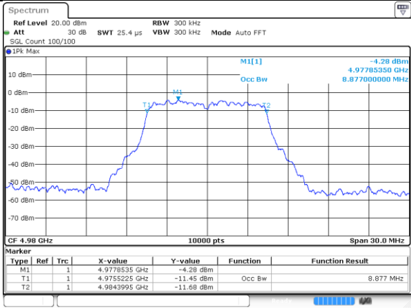
4980-10MHz-802.11ac-Radio_1
