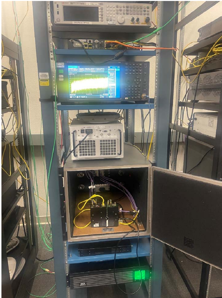
IW9165E-B & IW9165E-A Conducted test setup picture
