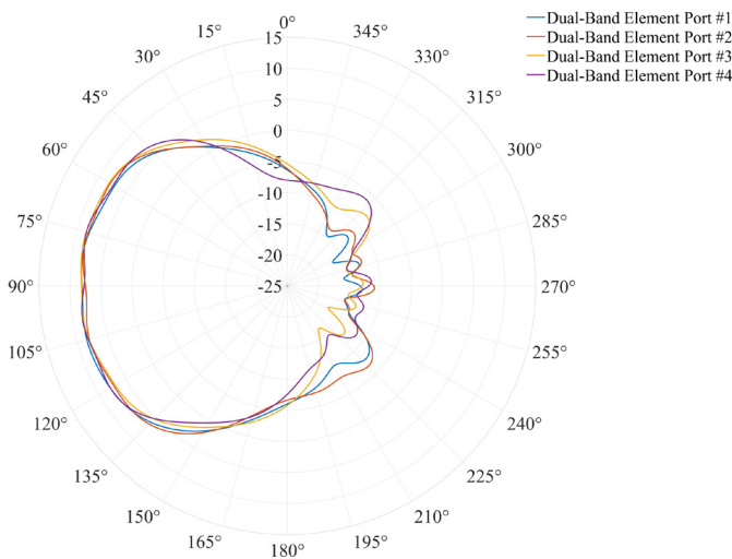
Azimuth Plane
