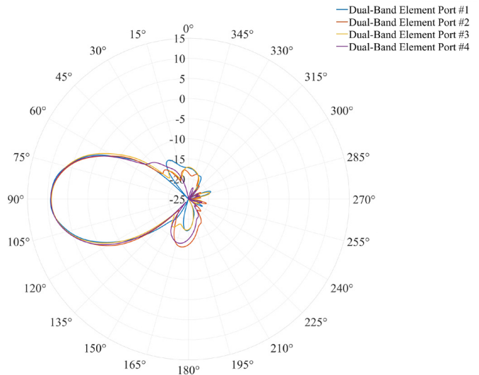
Elevation Plane
