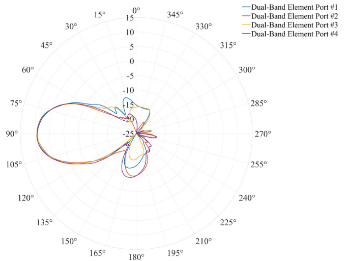
Elevation Plane
