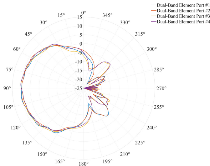
Azimuth Plane
