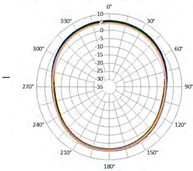
Azimuth Plane
