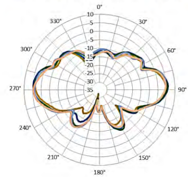
Phi 90° Plane
