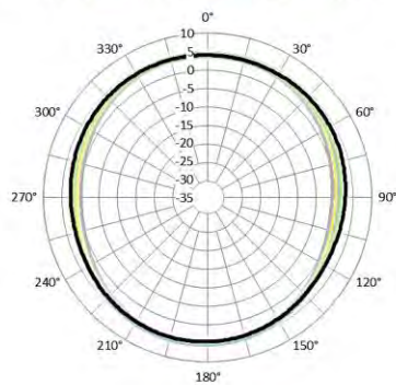
Azimuth Plane
