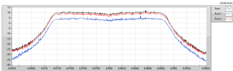
4.94-4.99GHz_11j.VHT20_20MHz_Nss1_2TX 4980MHz
