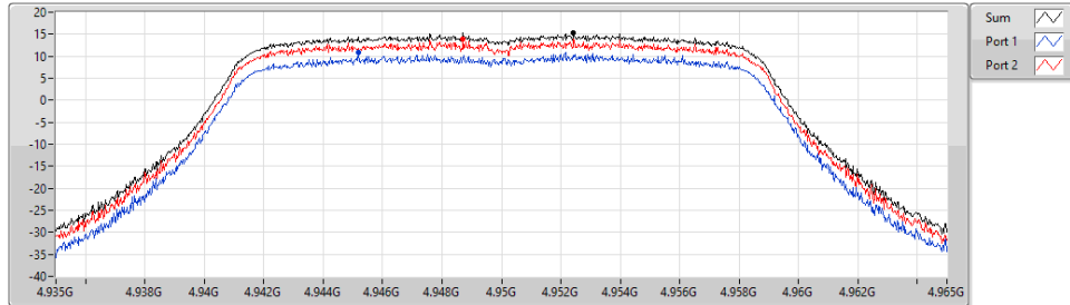
4.94-4.99GHz_11j.VHT20_20MHz_Nss1_2TX 4950MHz
