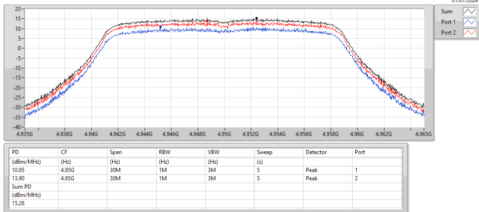
4.94-4.99GHz_11j.VHT20_20MHz_Nss1_2TX 4950MHz
