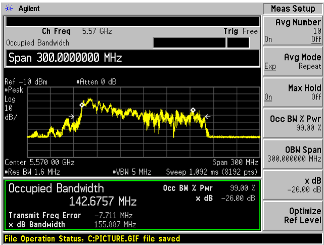
160 MHz
