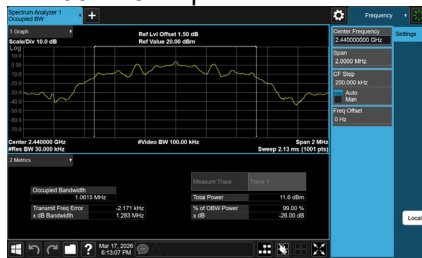
99 % Occupied Bandwidth
