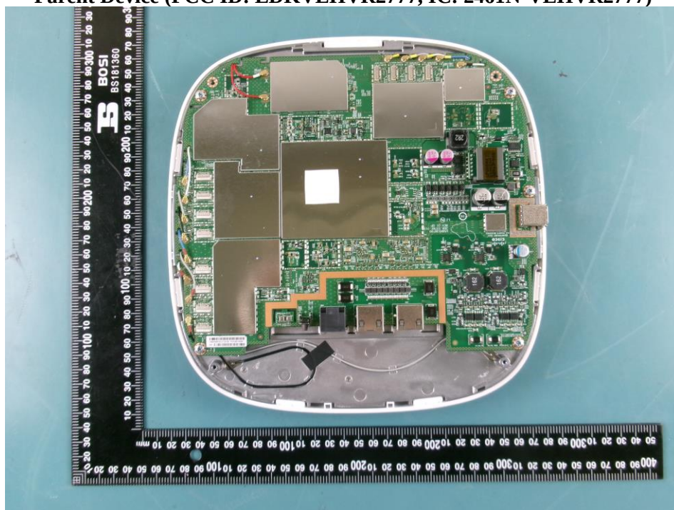
Parent Device (FCC ID: LDKVEHVR2777, IC: 2461N-VEHVR2777)
