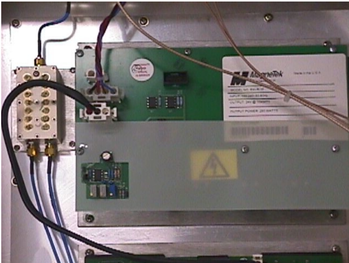
FIG 7. DUPLEXER (LEFT) FOR RX AND TX AND POWER MODULE
