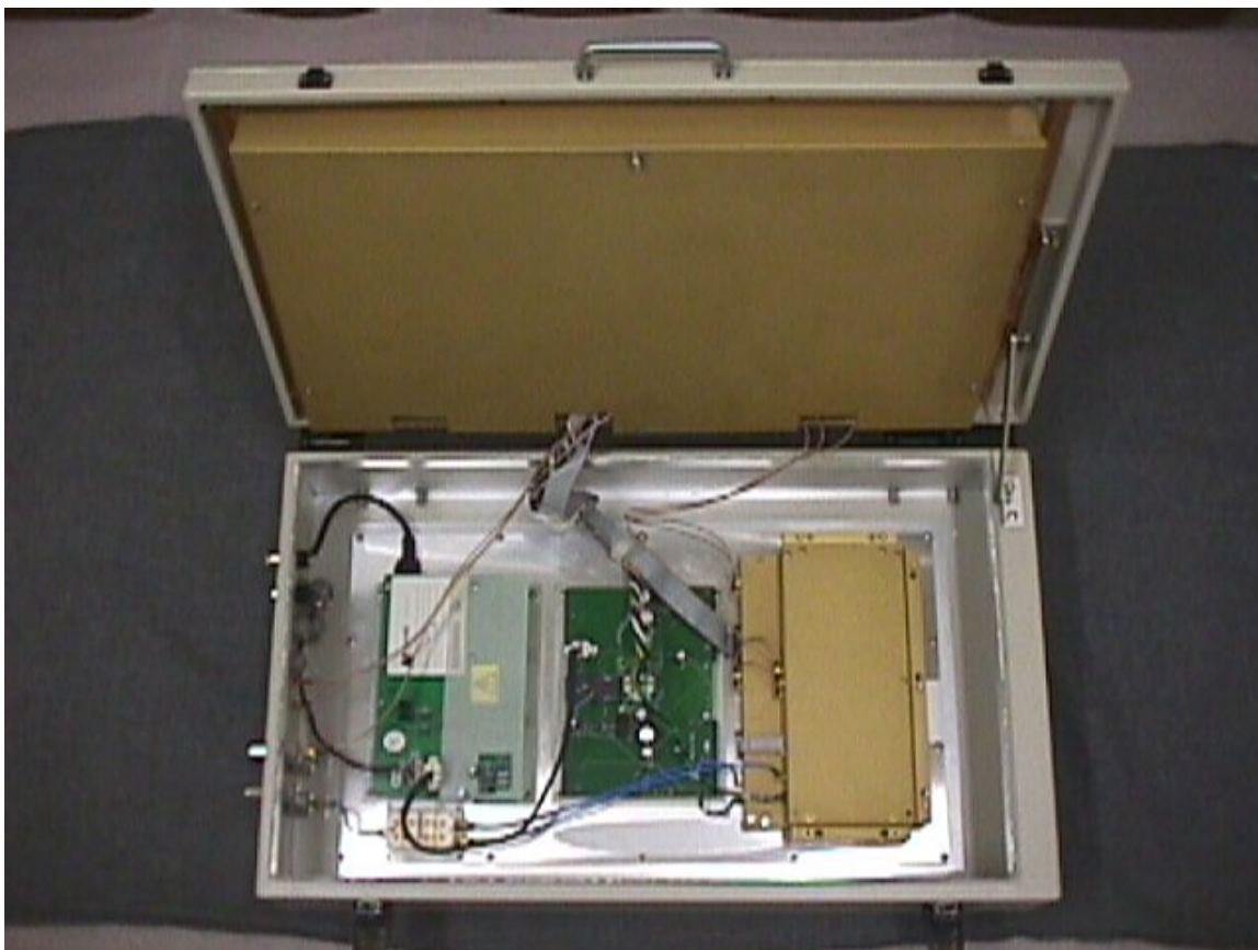
FIG 1. A PICTURE OF MWIBS SYSTEM OPENING FRONT DOOR
