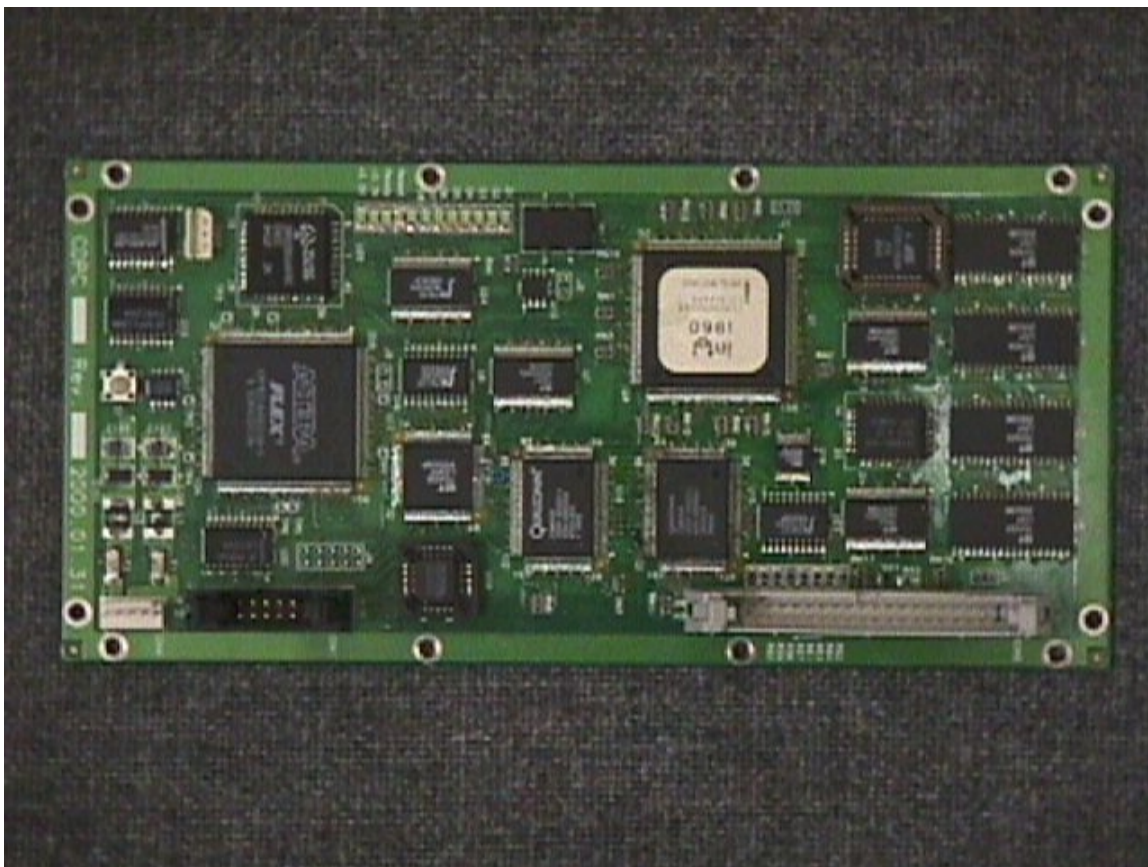
FIG 22. FRONTSIDE OF CHANNEL CARD BOARD (CDPC)
