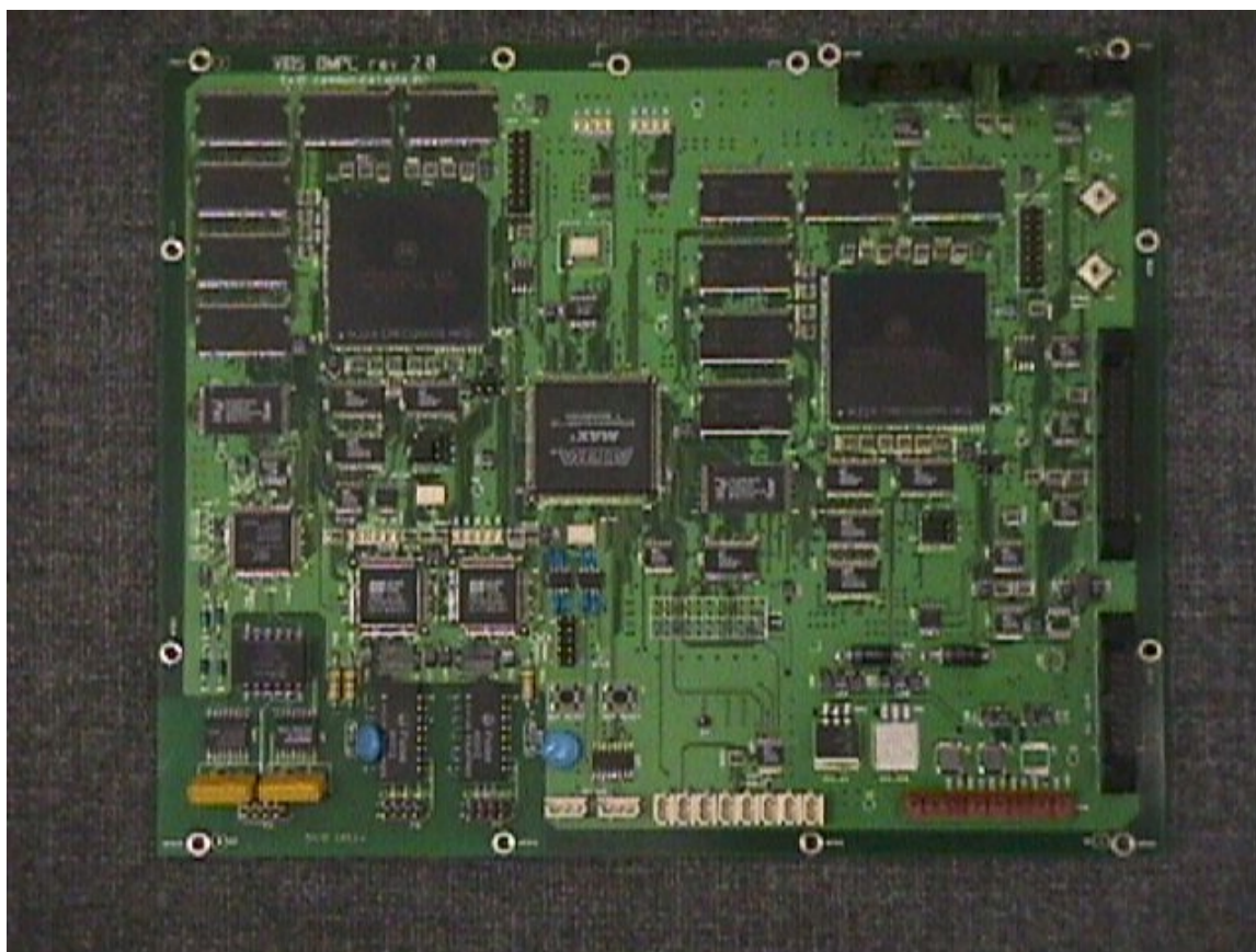
FIG 20. FRONT SIDE OF MAIN CONTROL BOARD (BMPC)
