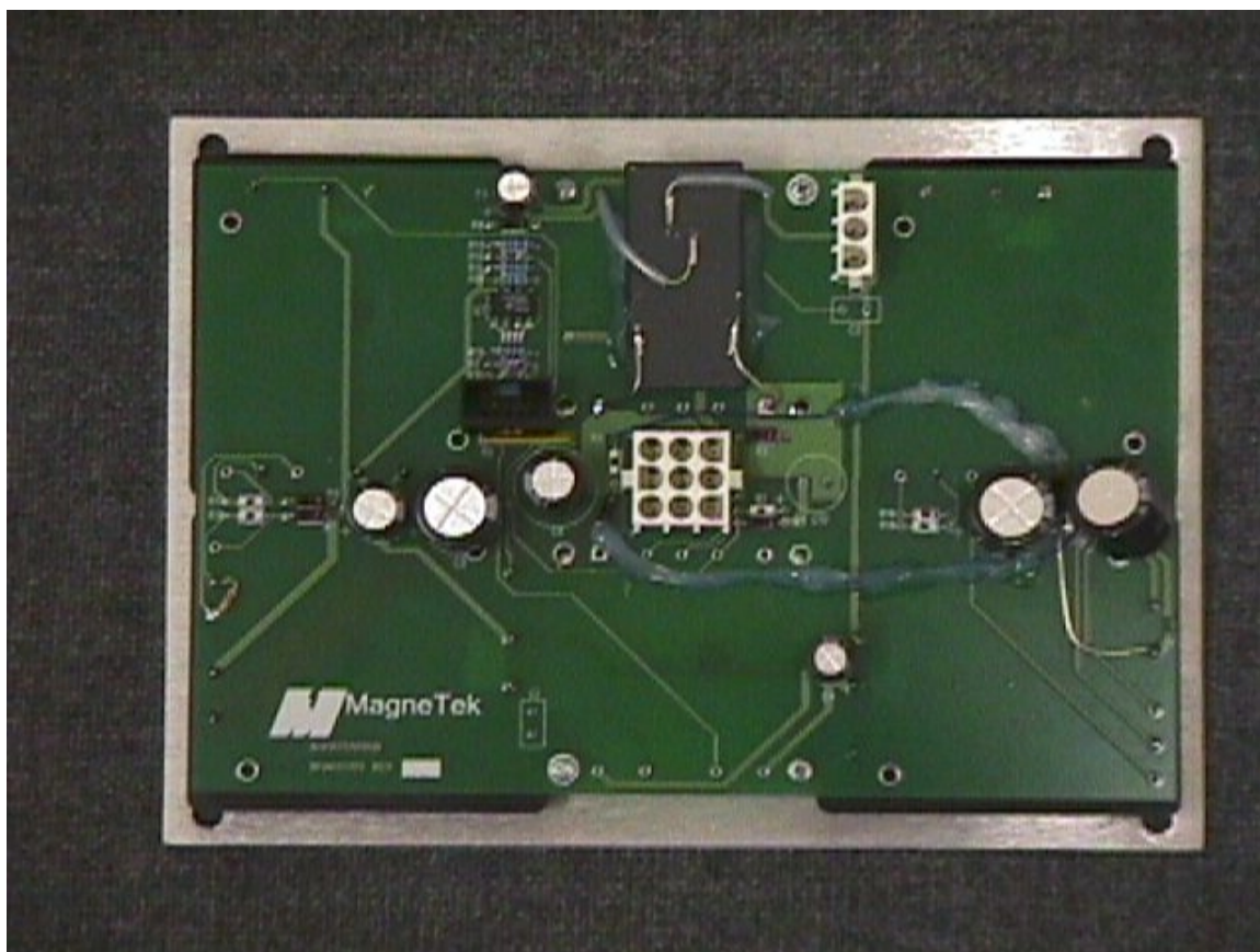
FIG 26. TOP VIEW OF POWER MODULE
