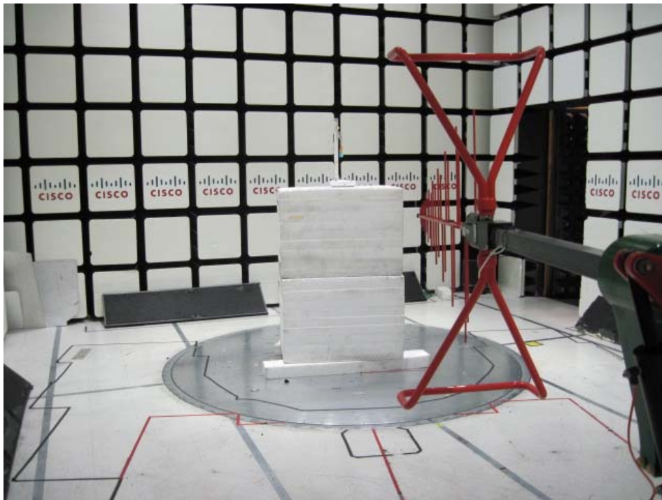
Title: Radiated Emissions Configuration Photograph 30MHz-1GHz
