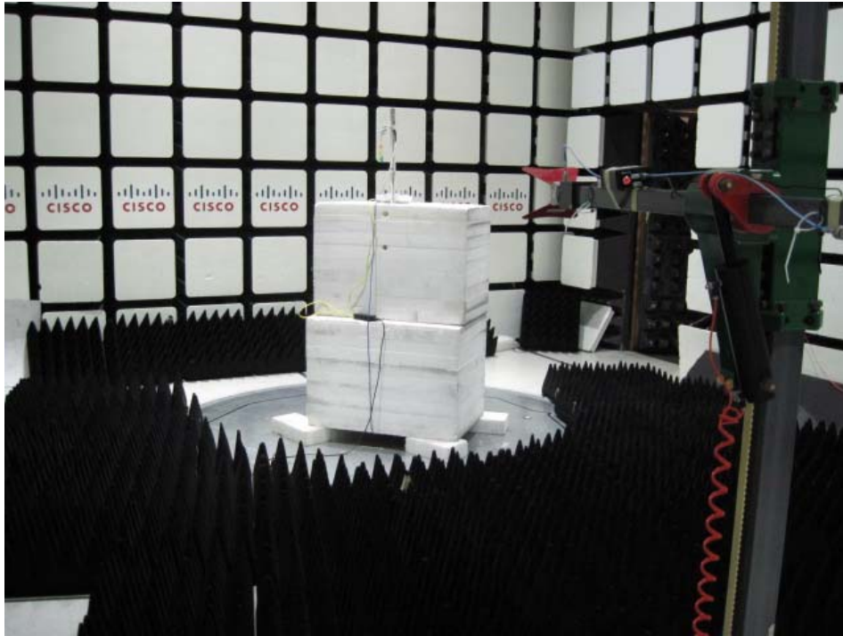
Title: Radiated Emissions Configuration Photograph 1-18GHz
