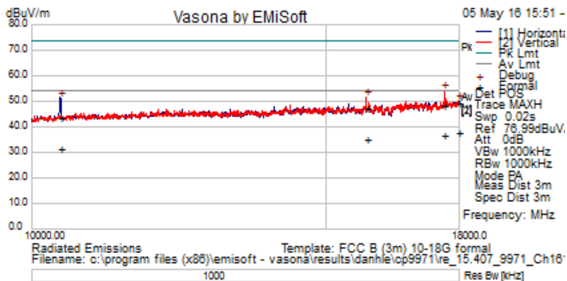
Title: TX Spurious Emissions from 10GHz-18GHz – Ch161 (5805 MHz)
