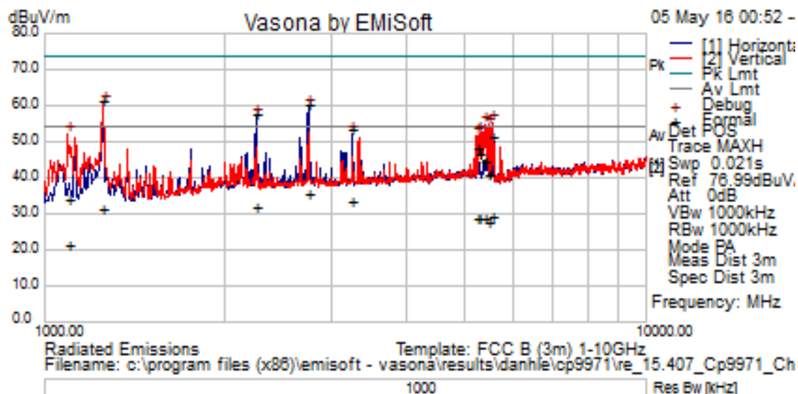
Title: TX Spurious Emissions from 1GHz-10GHz – Ch149 (5745 MHz)
