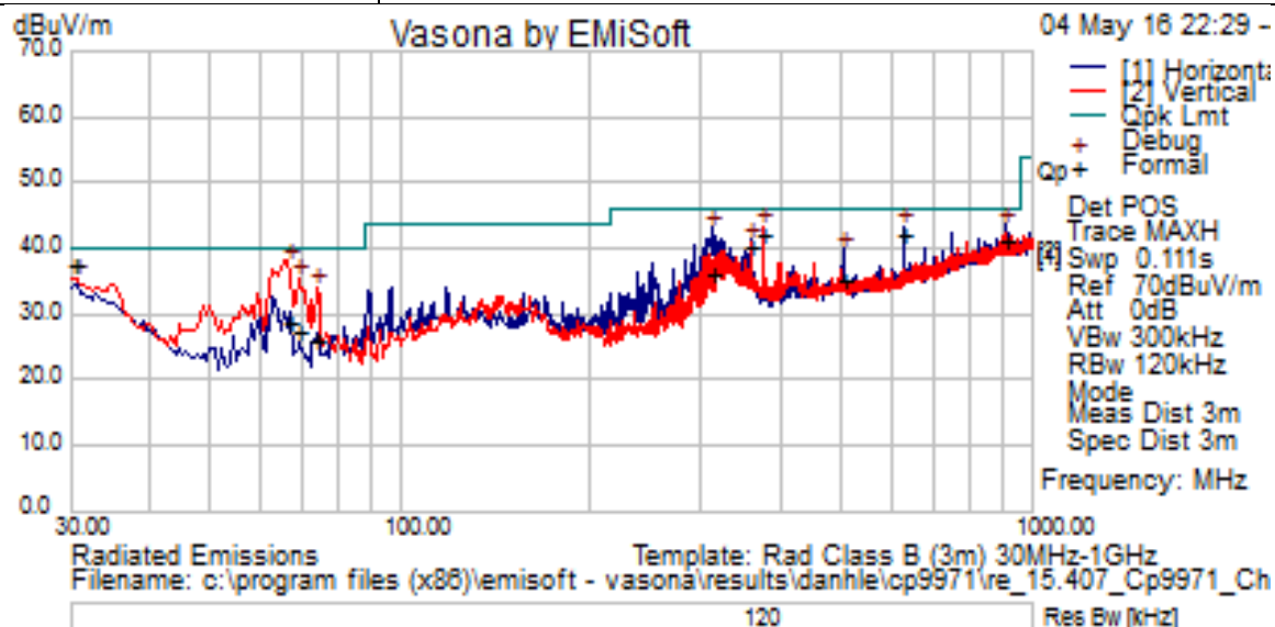
Title: TX Spurious Emissions from 30MHz-1GHz – Ch161 (5805 MHz)
