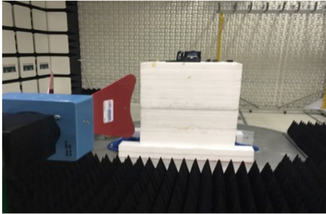
Title: Radiated Emissions Above 1 GHz
