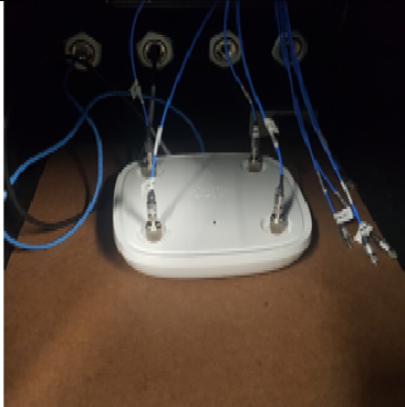
Conducted Test Setup Photo I
