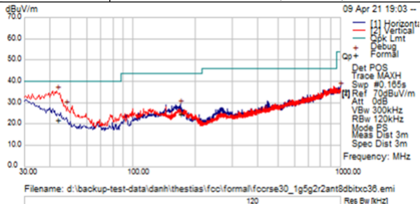
TX Spurious Emissions from 30MHz-1GHz – Ch36 (5180 MHz)
