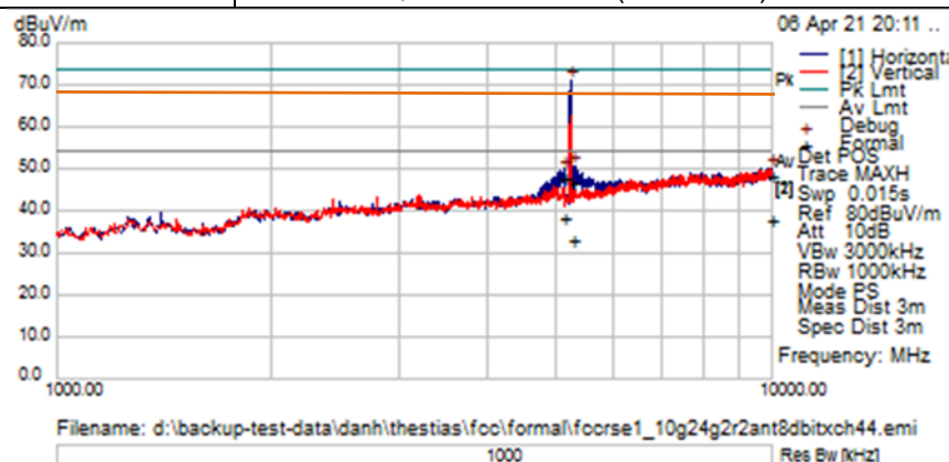
TX Spurious Emissions from 1GHz-10GHz – Ch44 (5220 MHz)
