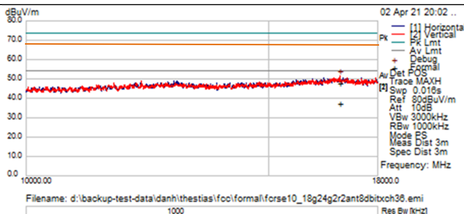
TX Spurious Emissions from 10GHz-18GHz – Ch36 (5180 MHz)
