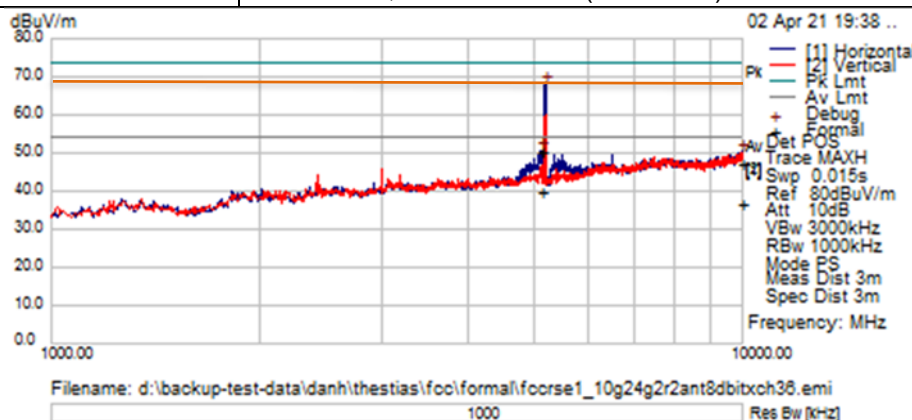
TX Spurious Emissions from 1GHz-10GHz – Ch36 (5180 MHz)
