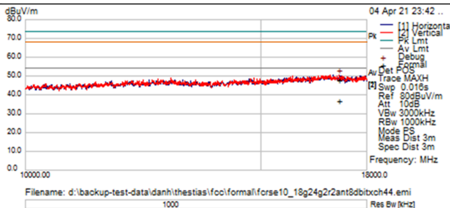
TX Spurious Emissions from 10GHz-18GHz – Ch44 (5220 MHz)
