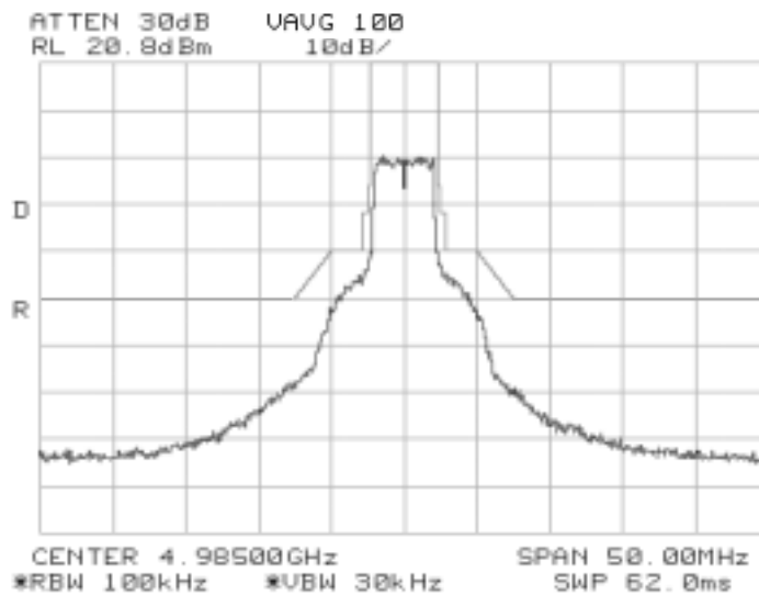
5MHz (4985 MHz)
