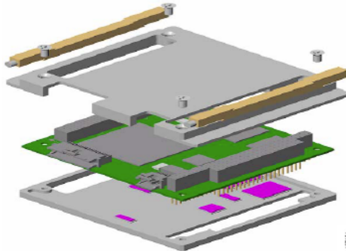
Figure 3 Exploded view of a Cisco 3200 Rugged Enclosure Card
