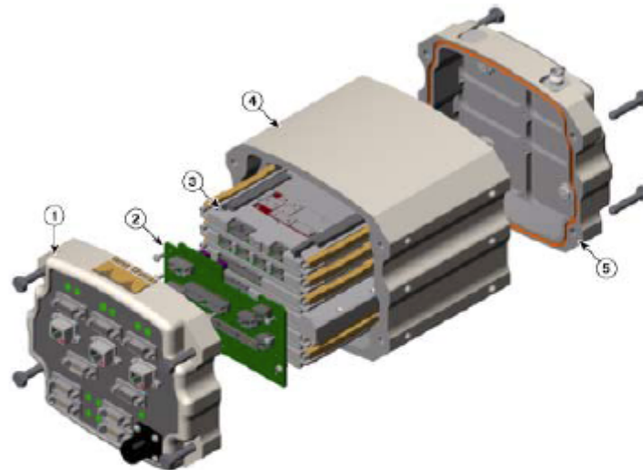
Figure 2 Exploded View of the Cisco 3200 Rugged Enclosure
