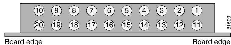
Figure 2-4 FESMIC LED Header Pin Locations
