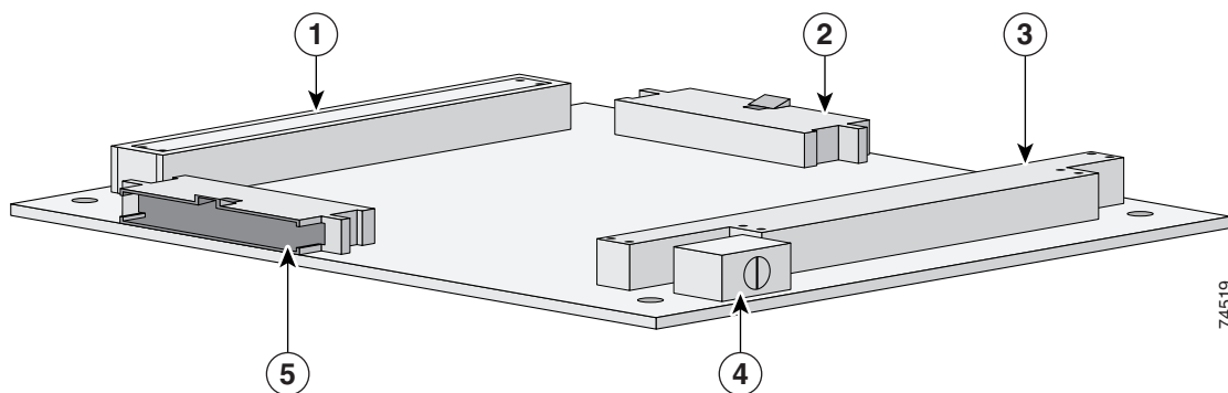
Figure 3-2 4-port SMIC Header and Bus Locations
