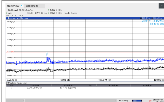
Radiated Emissions 7.75-12 GHz, Ch45, 802.11ax HT20 MIMO, HP
