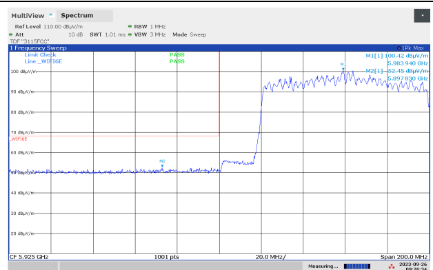
Band Edge, 5925 MHz, Ch07, 802.11ax HT80 MIMO, Pk, Max
