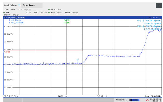
Band Edge, 5925 MHz, Ch03, 802.11ax HT40 MIMO, Pk, Max
