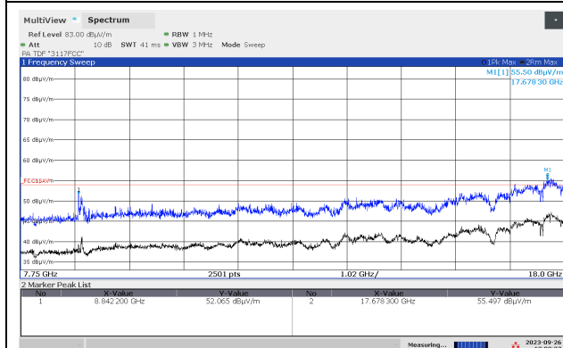
Radiated Emissions 7.75-18 GHz, Ch93, 802.11ax HT20 MIMO, HP
