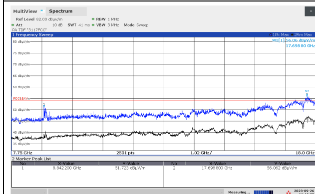
Radiated Emissions 7.75-18 GHz, Ch93, 802.11ax HT20 Ant1, HP
