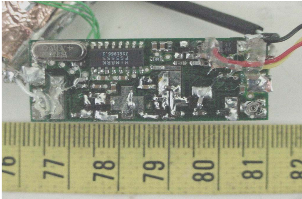
Component View of RF Module PCB
