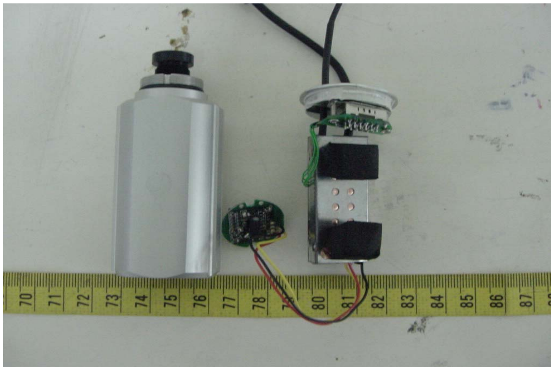
Internal View of Transmitter
