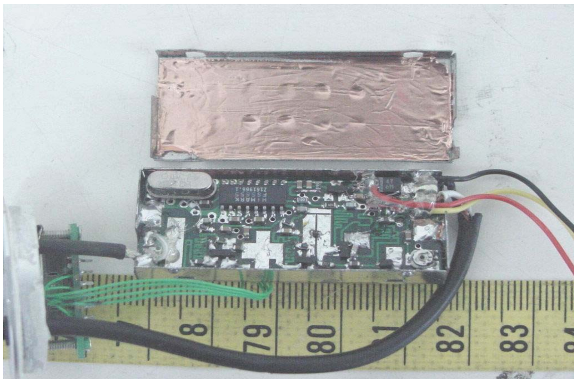
Internal View of RF Module
