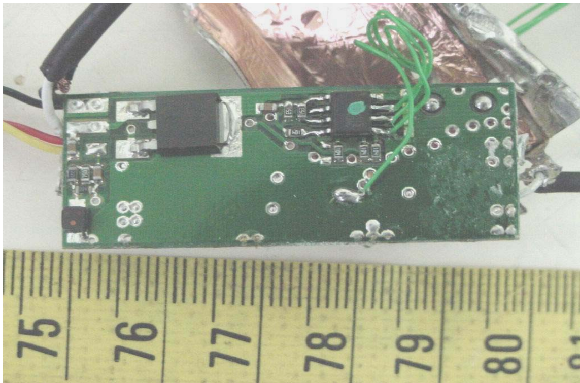
Solder View of RF Module PCB
