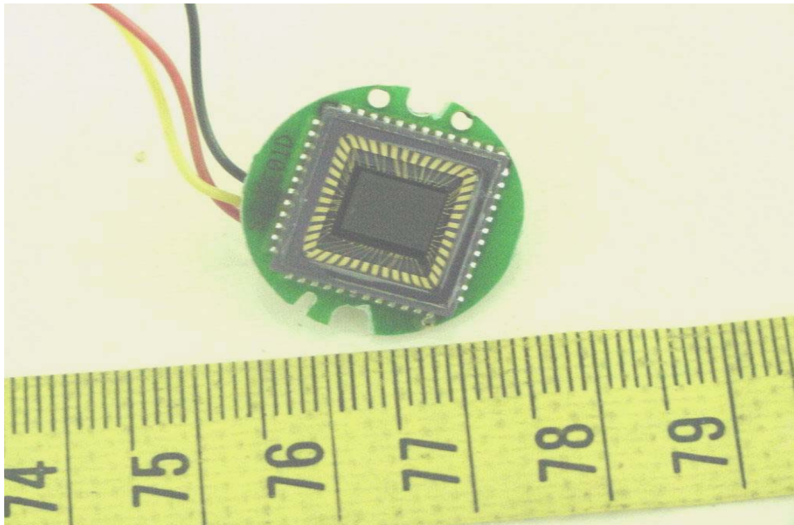
Component View of CCD PCB
