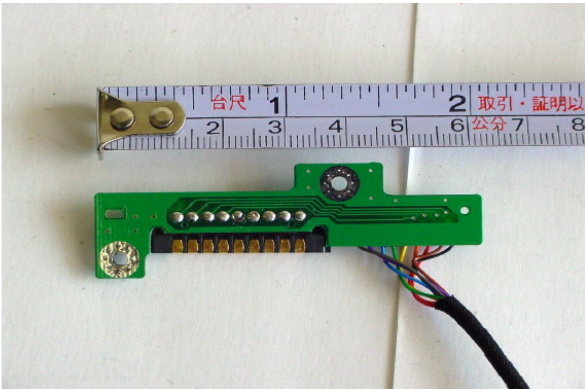
Solder View of Connected PCB
