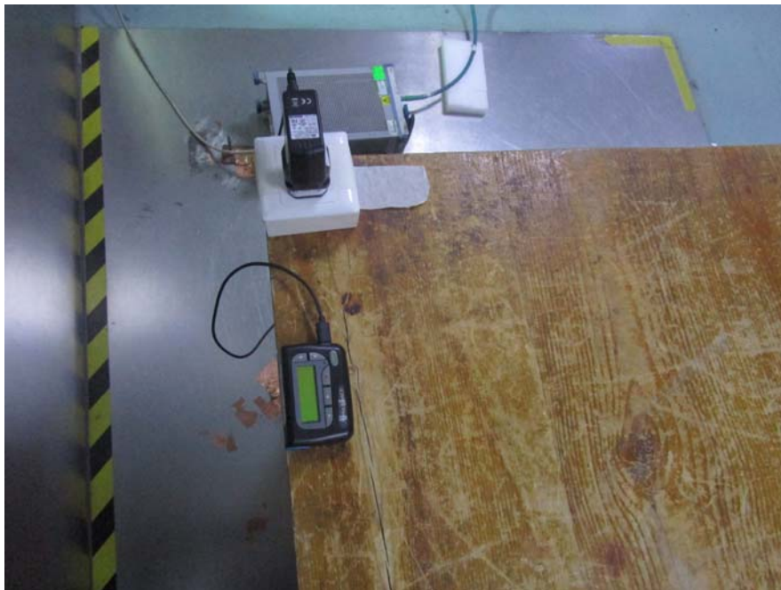
Conducted Emissions TM2– Side View
