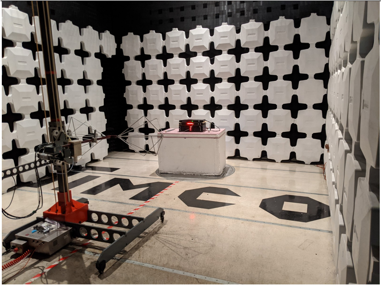
Radiated Unintentional Emissions, Below 1 GHz
