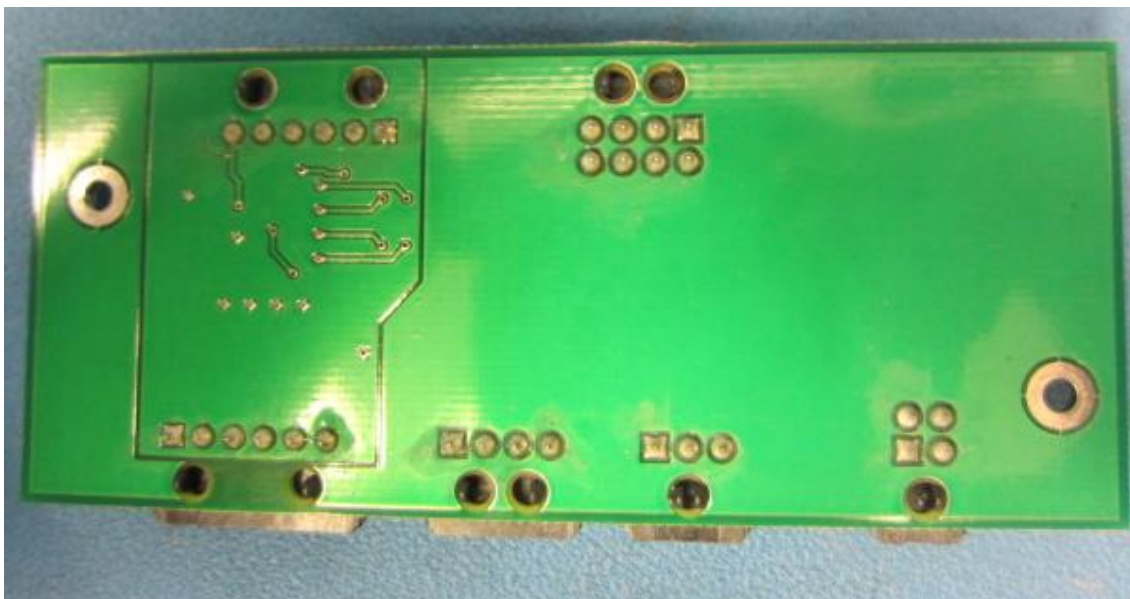
Figure 26 TX_Fan_PCB Bottom View
