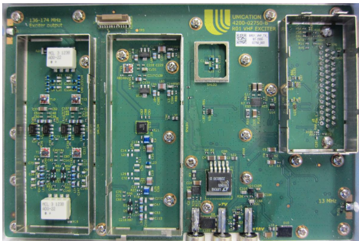
Figure 36 TX_EXciter_PCB Top View
