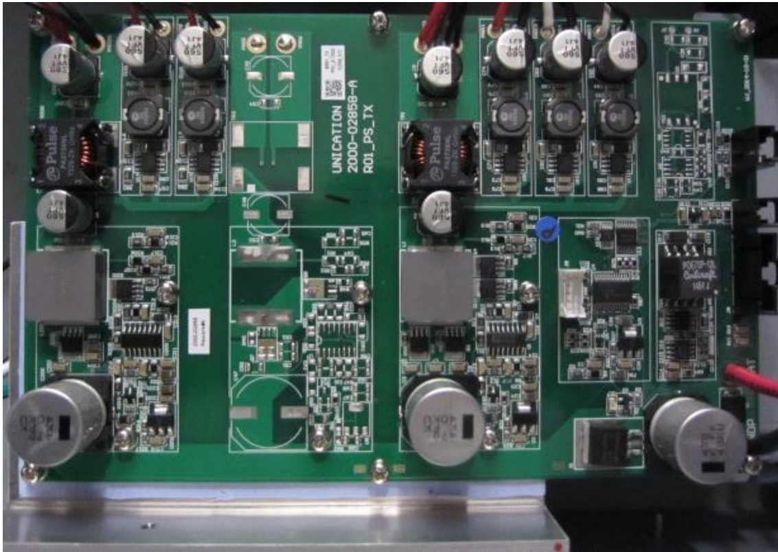
Figure 23 TX_PSU_PCB Top View
