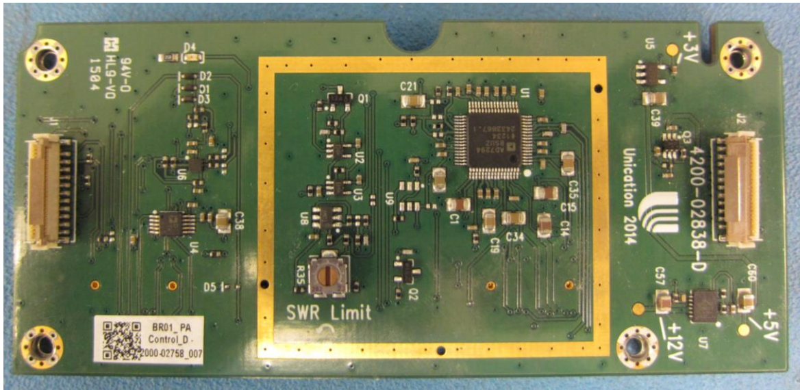
Figure 32 TX_PA_CTRL_PCB Top View
