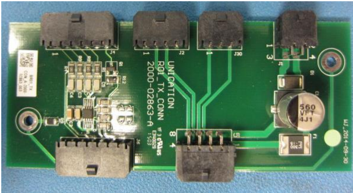
Figure 25 TX_Fan_PCB Top View
