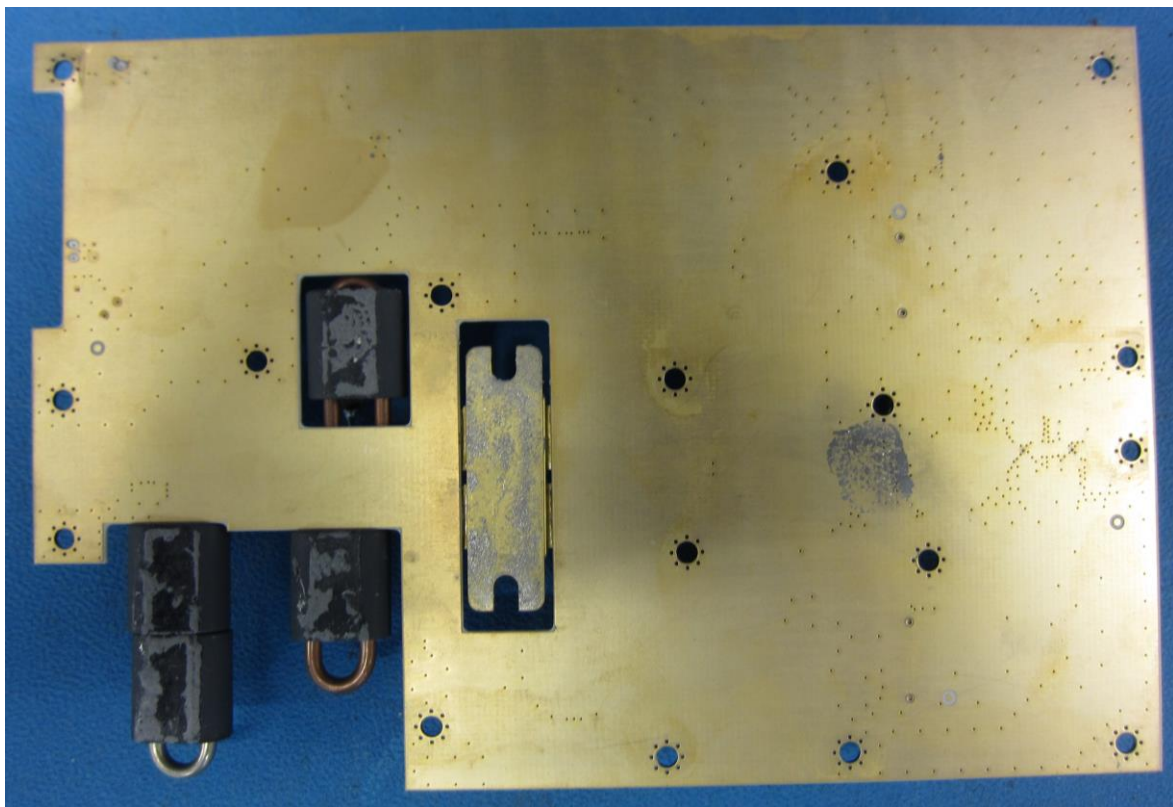
Figure 31 TX_PA_PCB Bottom View
