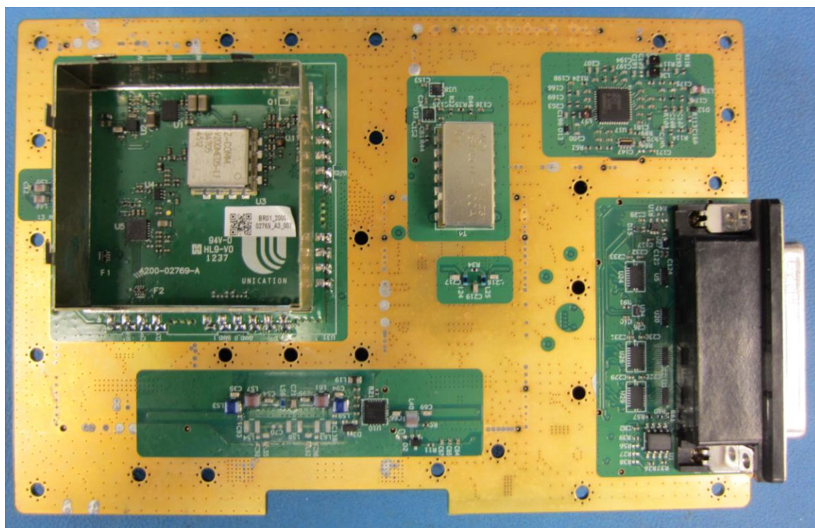
Figure 37 TX_EXciter_PCB Bottom View
