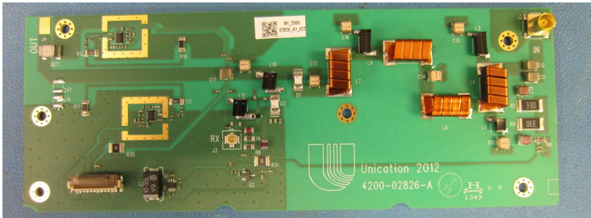
Figure 34 TX_OUTPUT_Filter_PCB Top View
