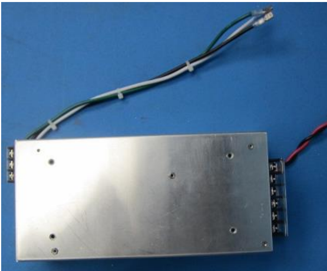
Figure 40 TX_Meanswell_PSU Bottom View
