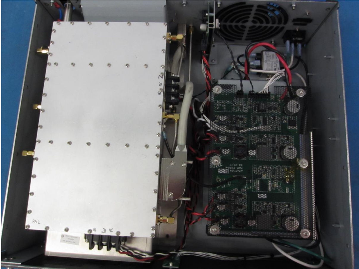
Figure 43 TX_Chassis Top View
