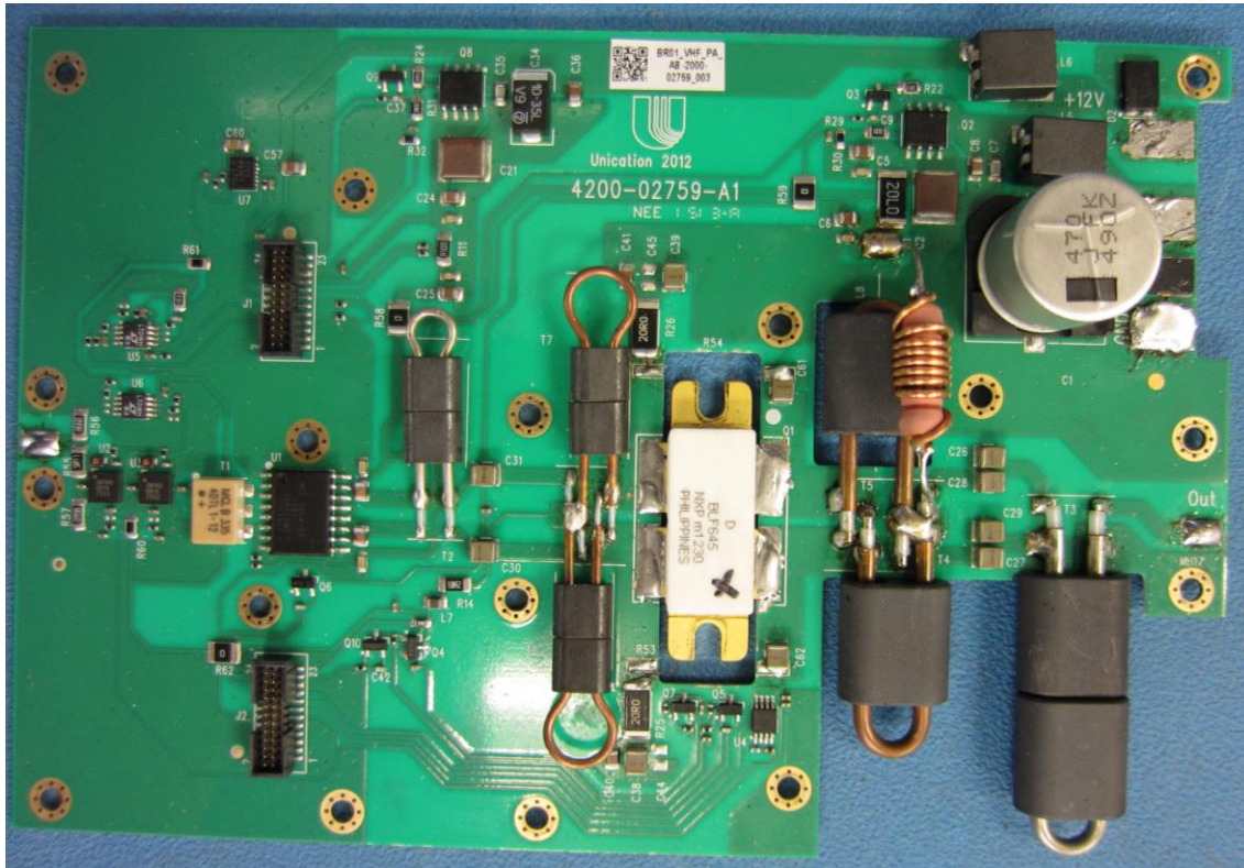
Figure 30 TX_PA_PCB Top View
