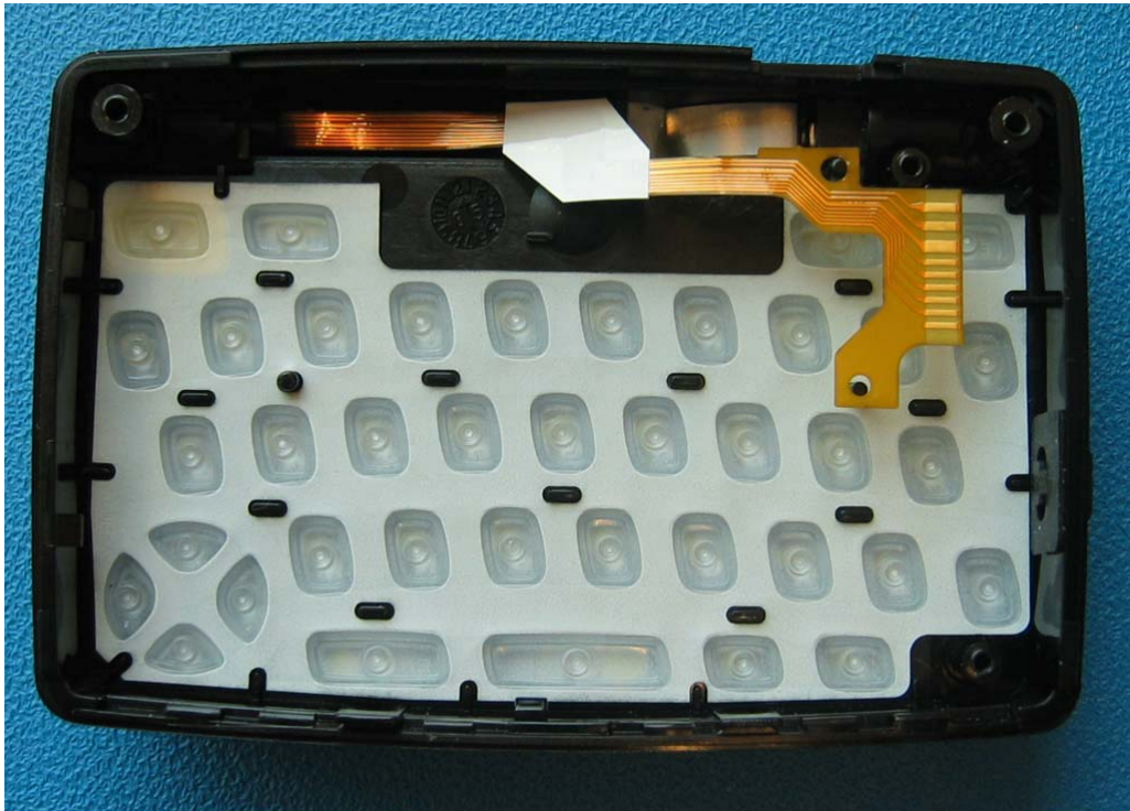
VIEW OF KEYBOARD - BOTTOM
