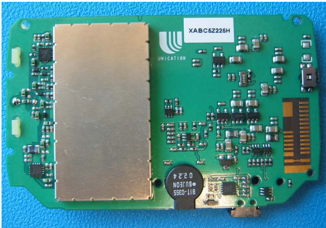
VIEW OF MAIN BOTTOM WITH SHIELD
