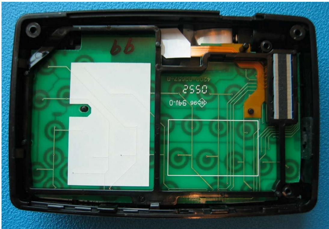
VIEW OF KEYBOARD - SPACER
