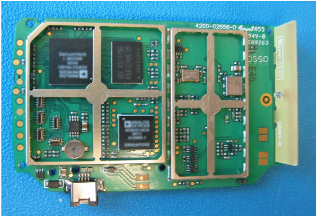
VIEW OF MAIN PCB TOP
