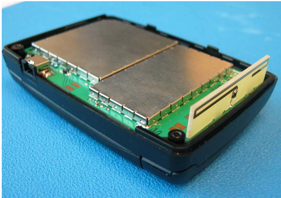
VIEW OF INTERNAL ANTENNA
