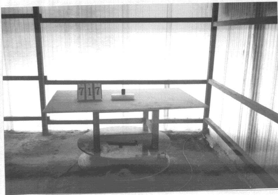
Fig 2. Test Configuration of the Radiated Emissions (Back View)
