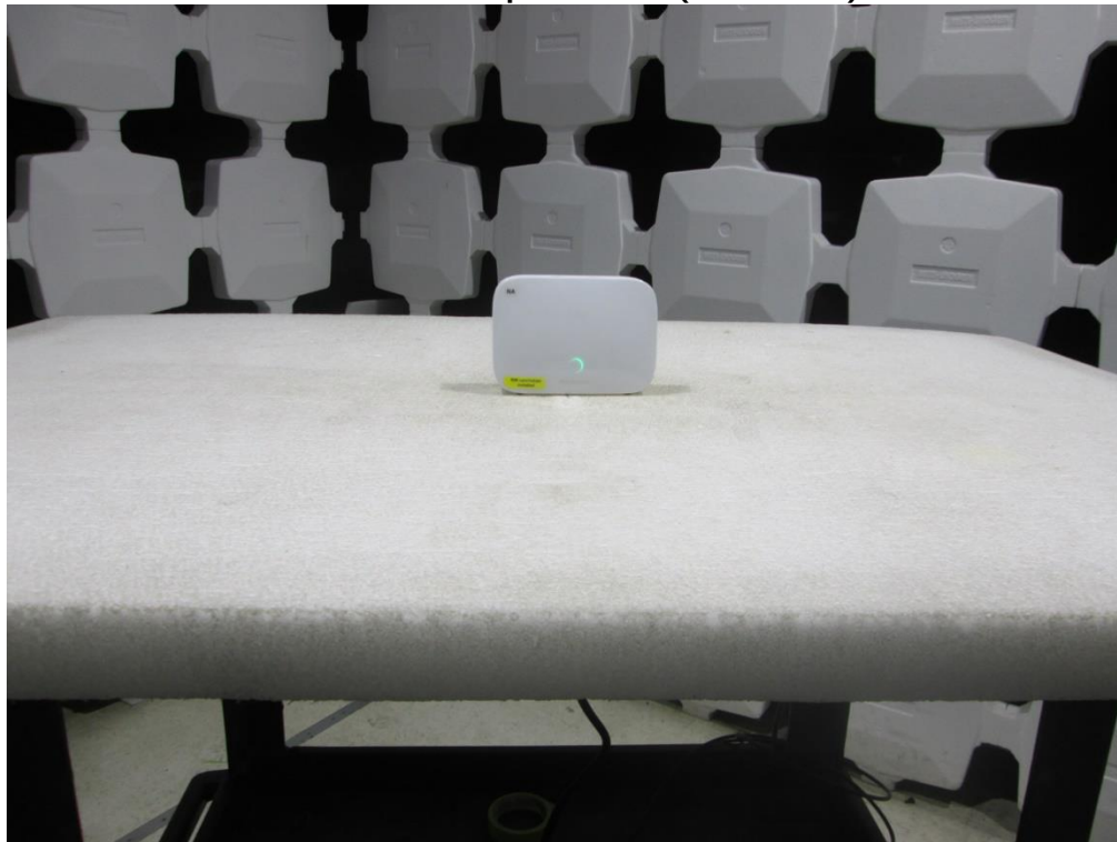
Radiated Spurious (Vertical)
