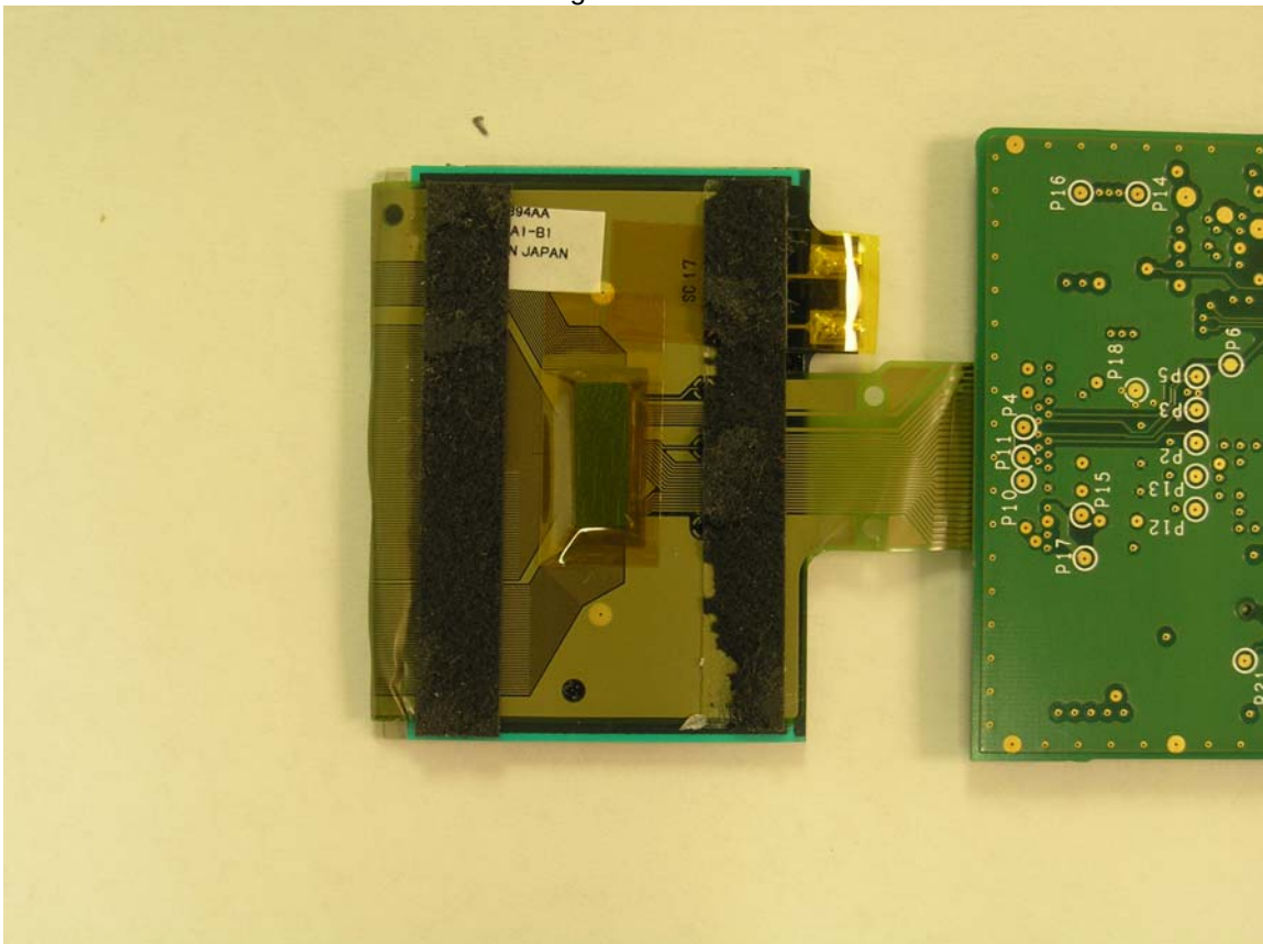
Patient Programmer - LCD Back
