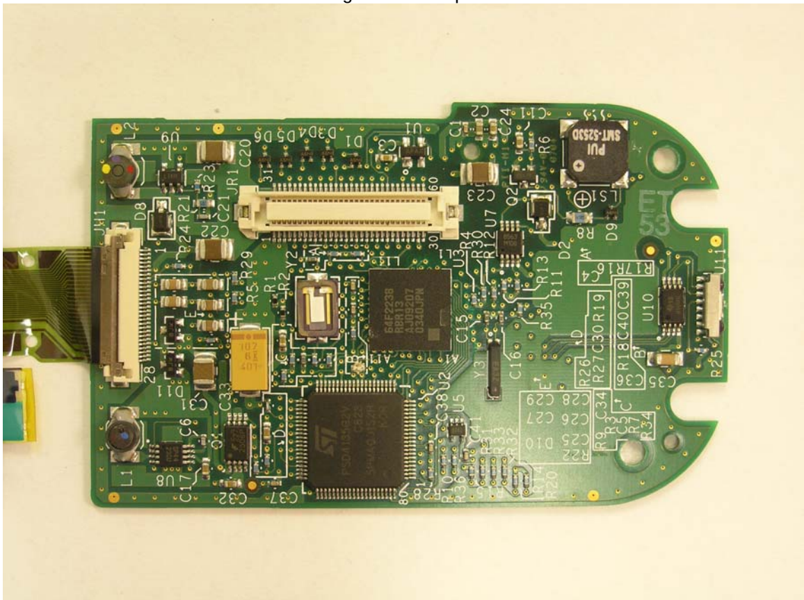
Patient Programmer - Top of Board 1
