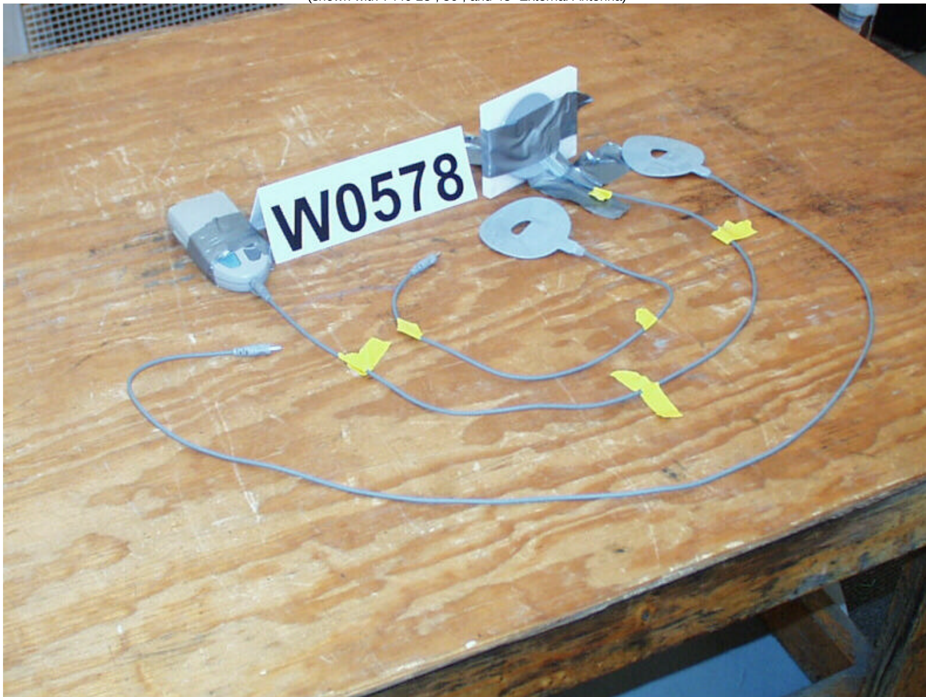
7434A Patient Programmer (representative of Models 3031A and 7438) Radiated Emissions Test Setup (shown with 7440 23", 36", and 48" External Antenna)
