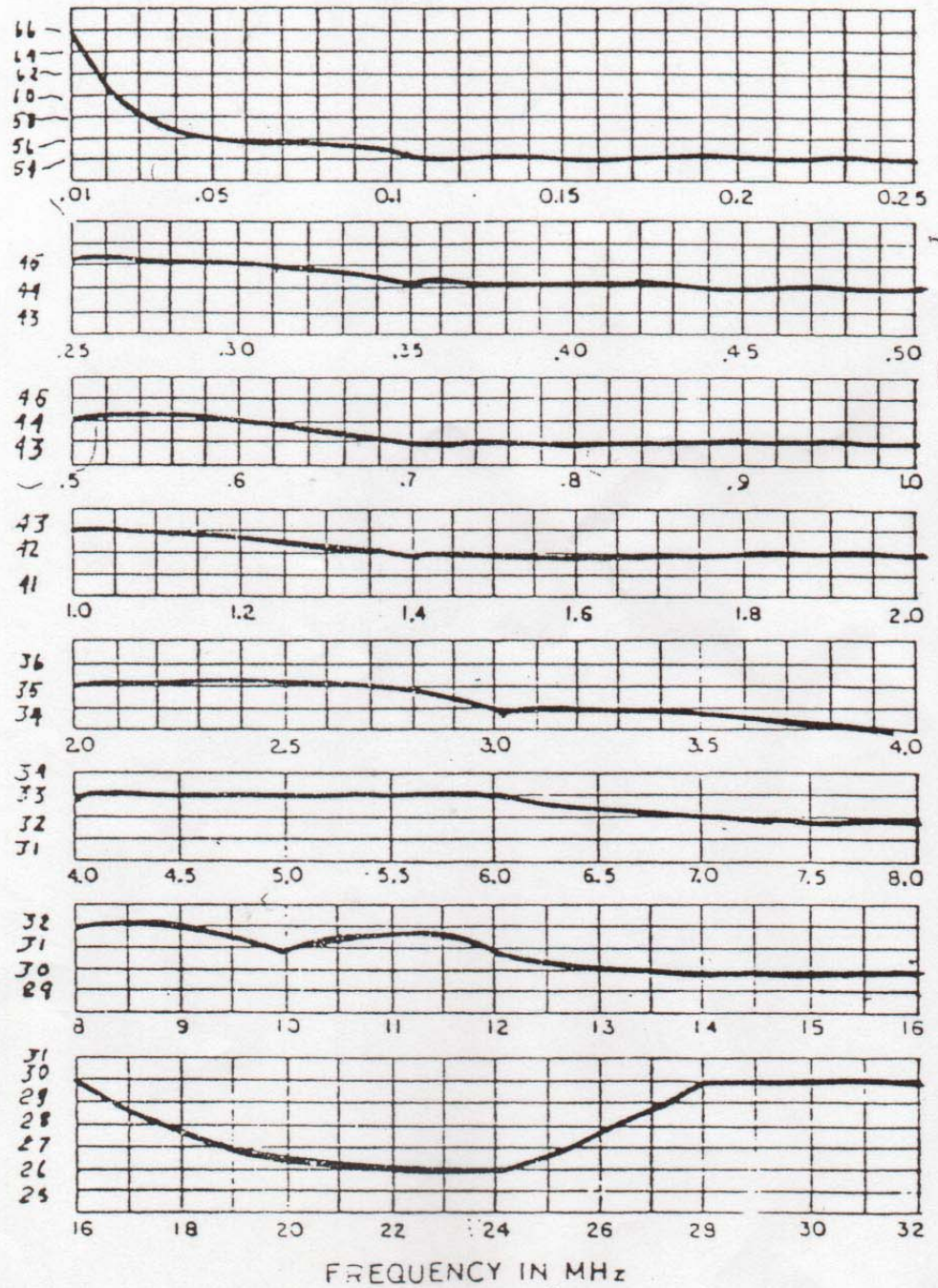
LOOP ANTENNA CORRECTION FACTORS IN dB
