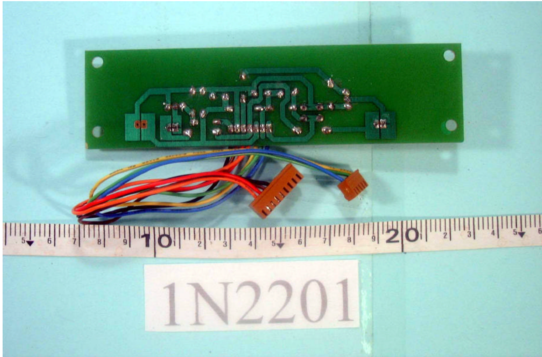
REAR SIDE Control panel board
