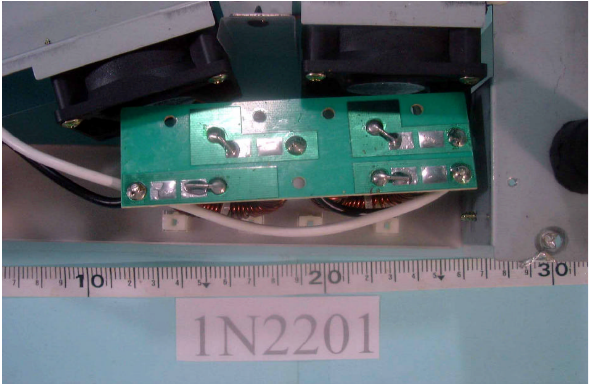
REAR SIDE Module board
