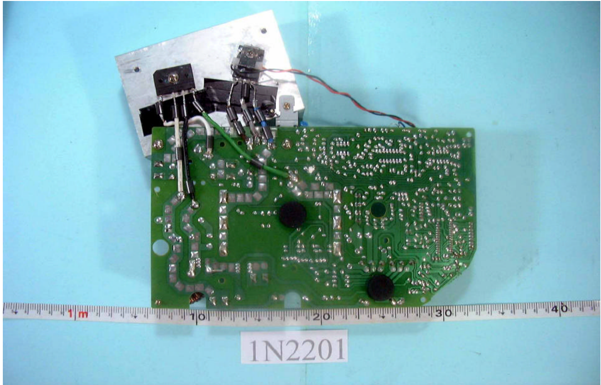
REAR SIDE Main board
