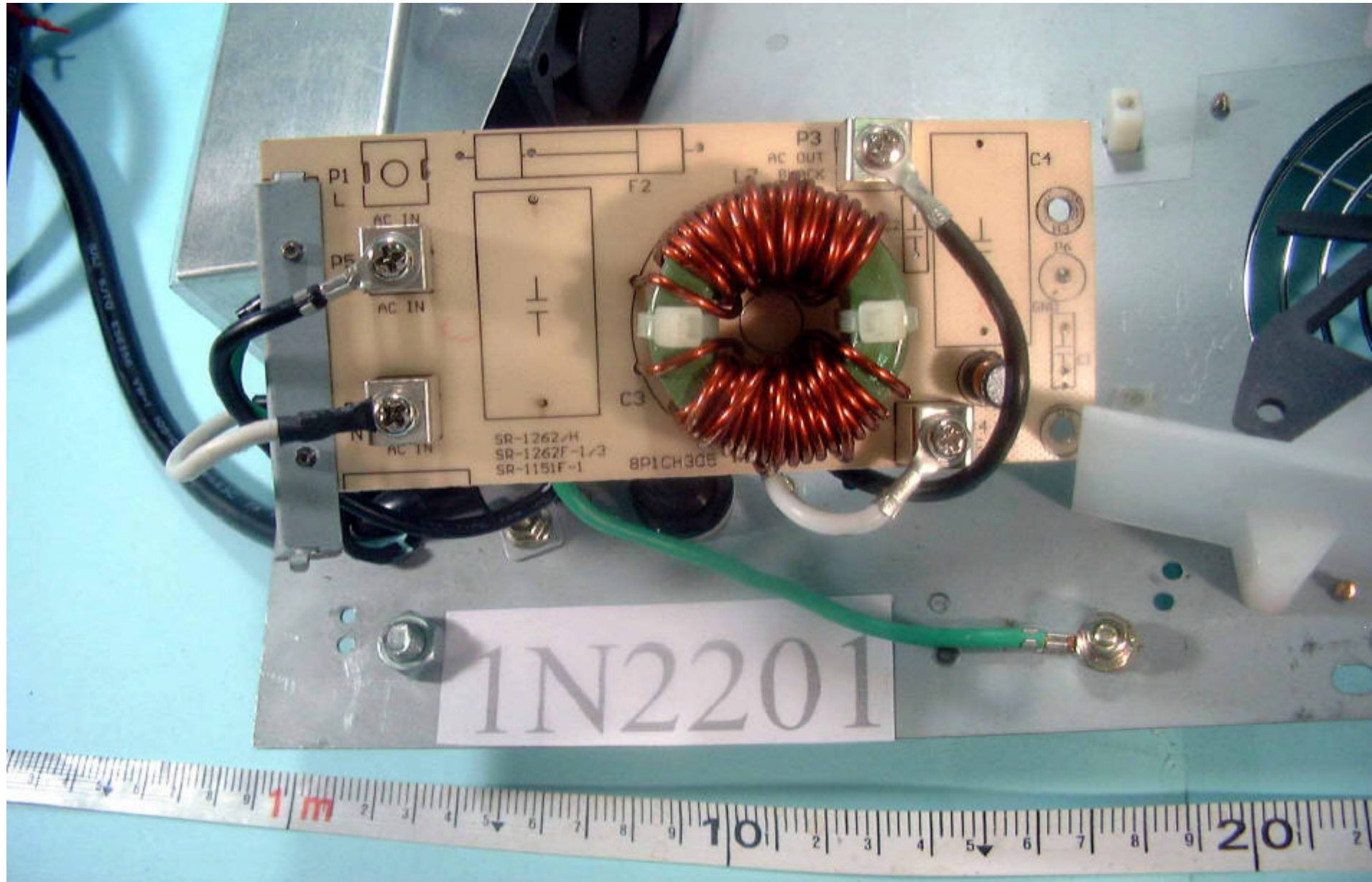
Front SIDE Module board
