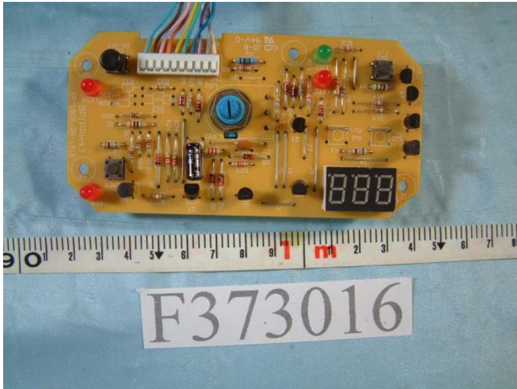
FRONT SIDE of CONTROL PANEL BOARD
