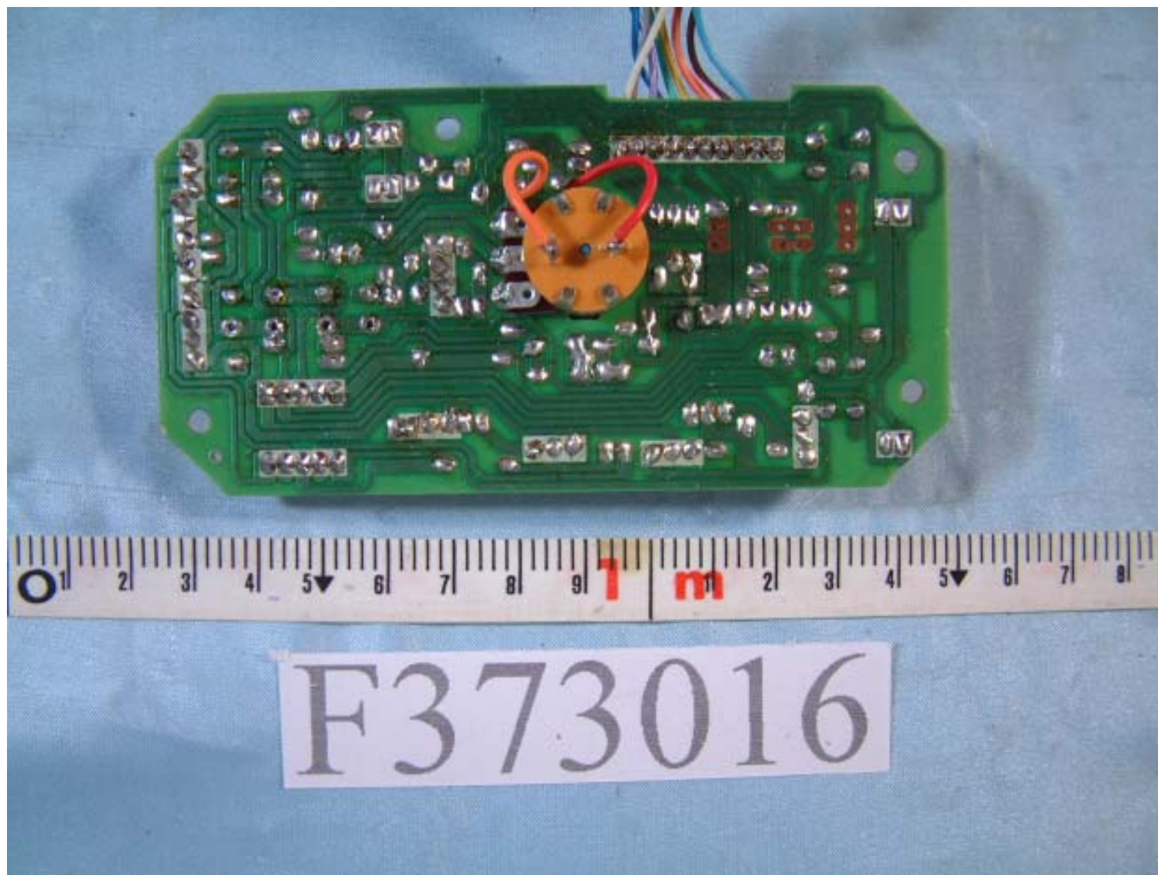
REAR SIDE of CONTROL PANEL BOARD
