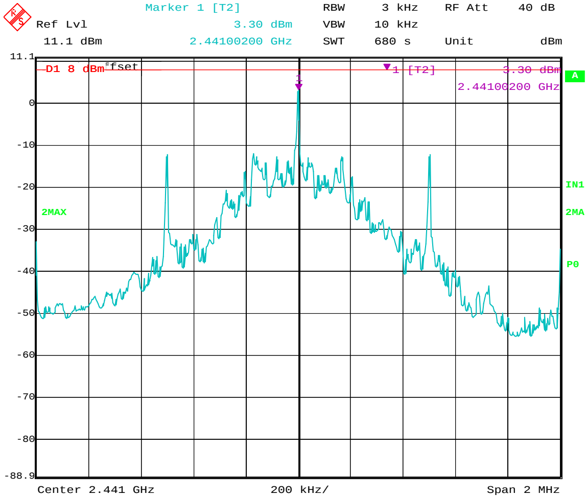
Spectral Density Output – Middle Channel
