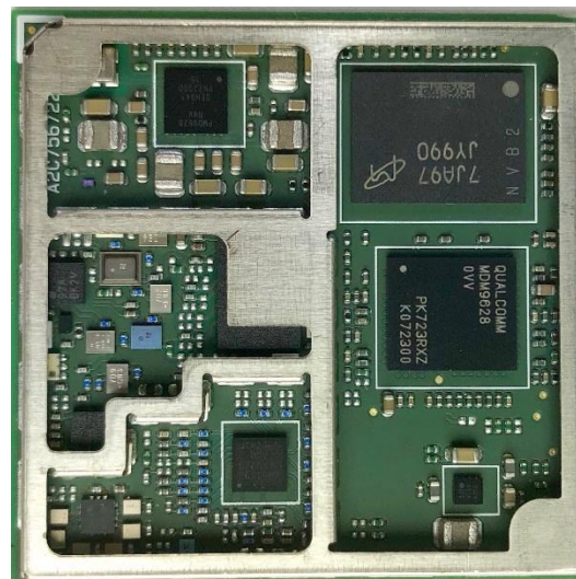
Fig. 2. BL28NA-001 top view with the shield removed.
