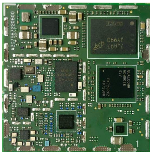
Fig. 3. BL28NA-001 module top view with the shield and shield frame removed.
