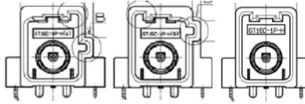
RF Connector – pin details (View from mating side)
