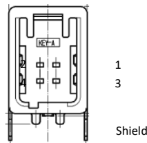
USB Connector – pin details (View from mating side)
