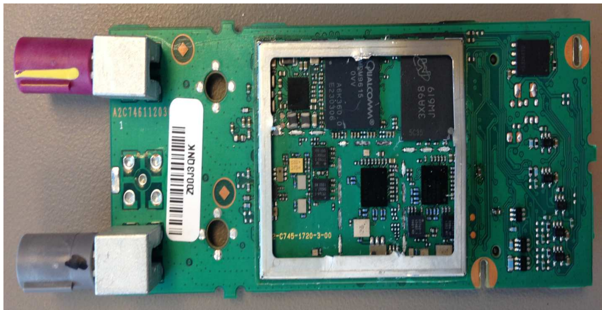
Internal view with internal shield removed
