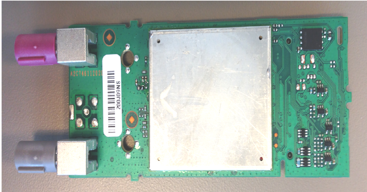
Top View without external shields
