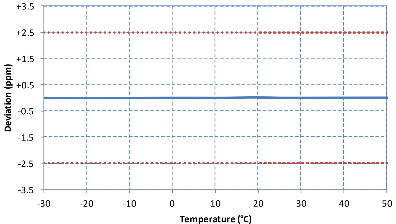
Frequency Stability
