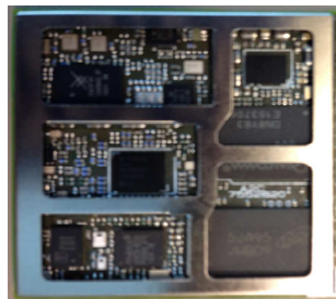
Fig. 2. FANW view without shield
