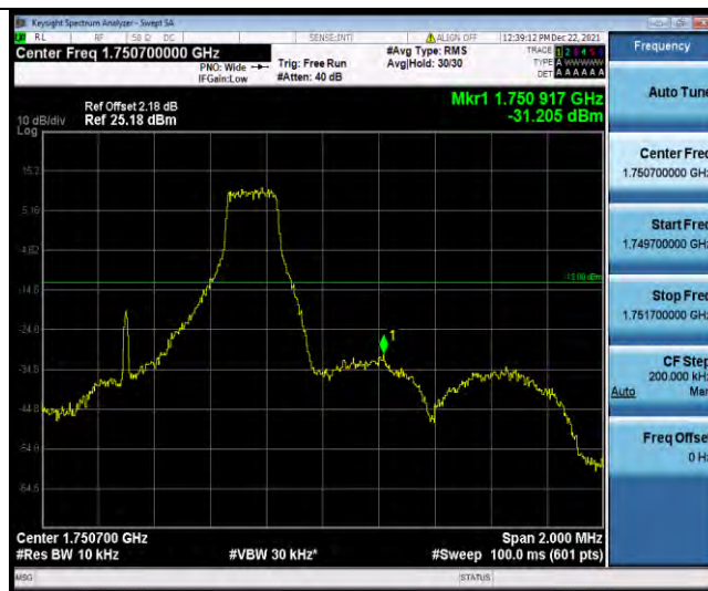
Band4-1.4MHz-QPSK-20350-6RB#0
